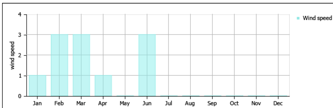
Figure 3.1.6: Average wind speed over the year in Cox's Bazar 4
