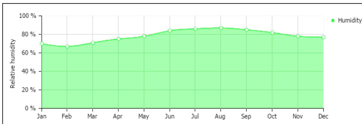
Figure 3.1.5: Average humidity over the year in Cox's Bazar 3
