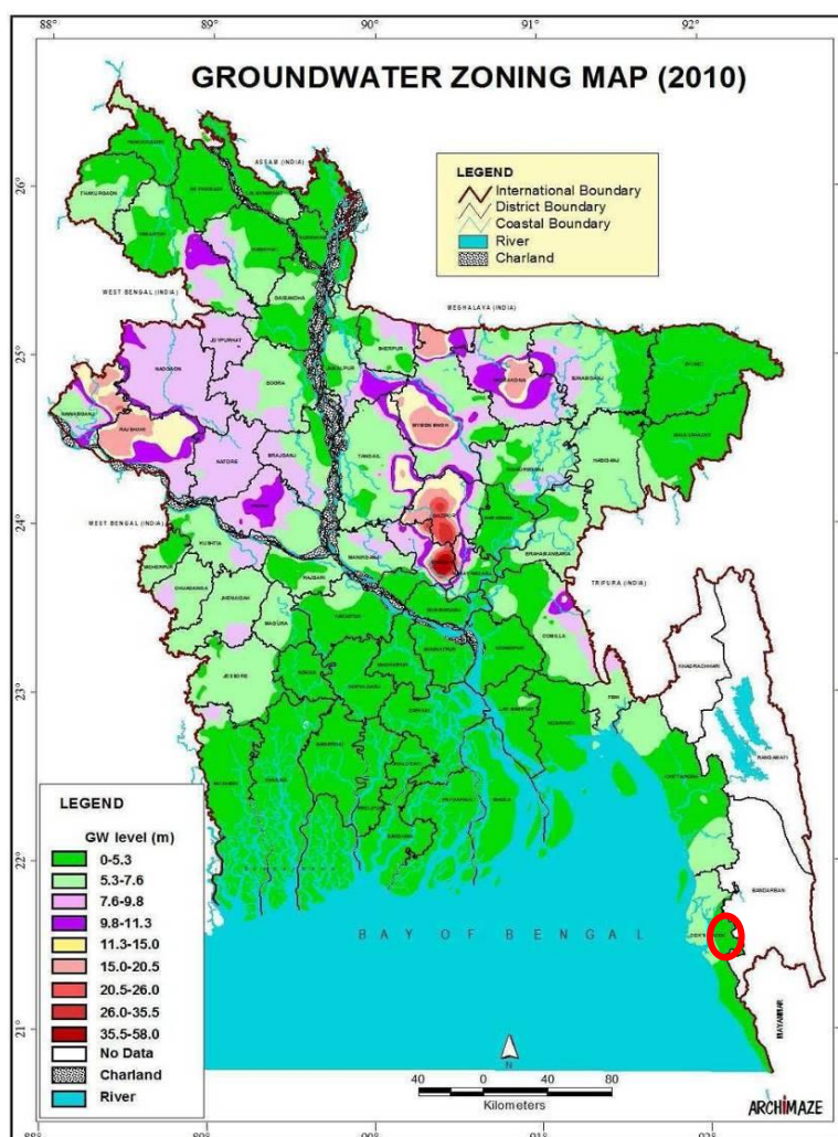
Figure 3.1.8: Location of Cox's Bazar Pourashava in Groundwater Zoning Map of Bangladesh
