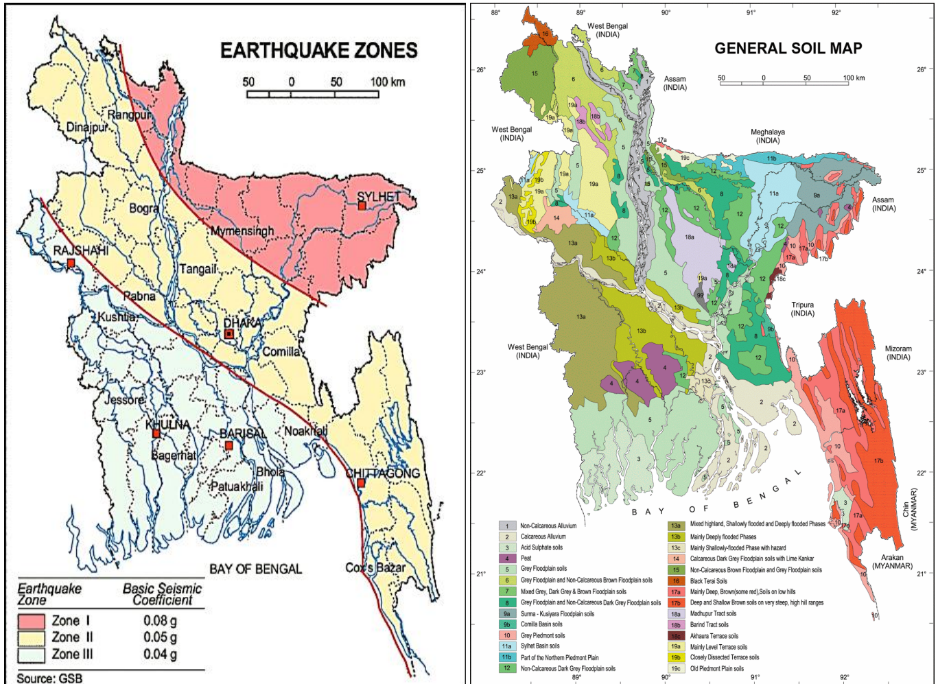
Figure 3.1.1: Location of Cox's Bazar Pourashava in Earthquake Zoning map of Bangladesh and general soil map of Bangladesh
