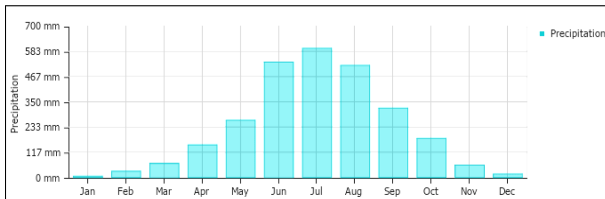
Figure 3.1.4: Average monthly Precipitation (Rainfall pattern) in Cox's Bazar 2
