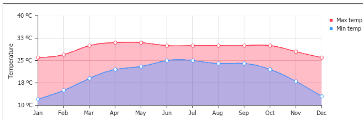
Figure 3.1.3: Average Minimum and Maximum Temperature in Cox's Bazar
