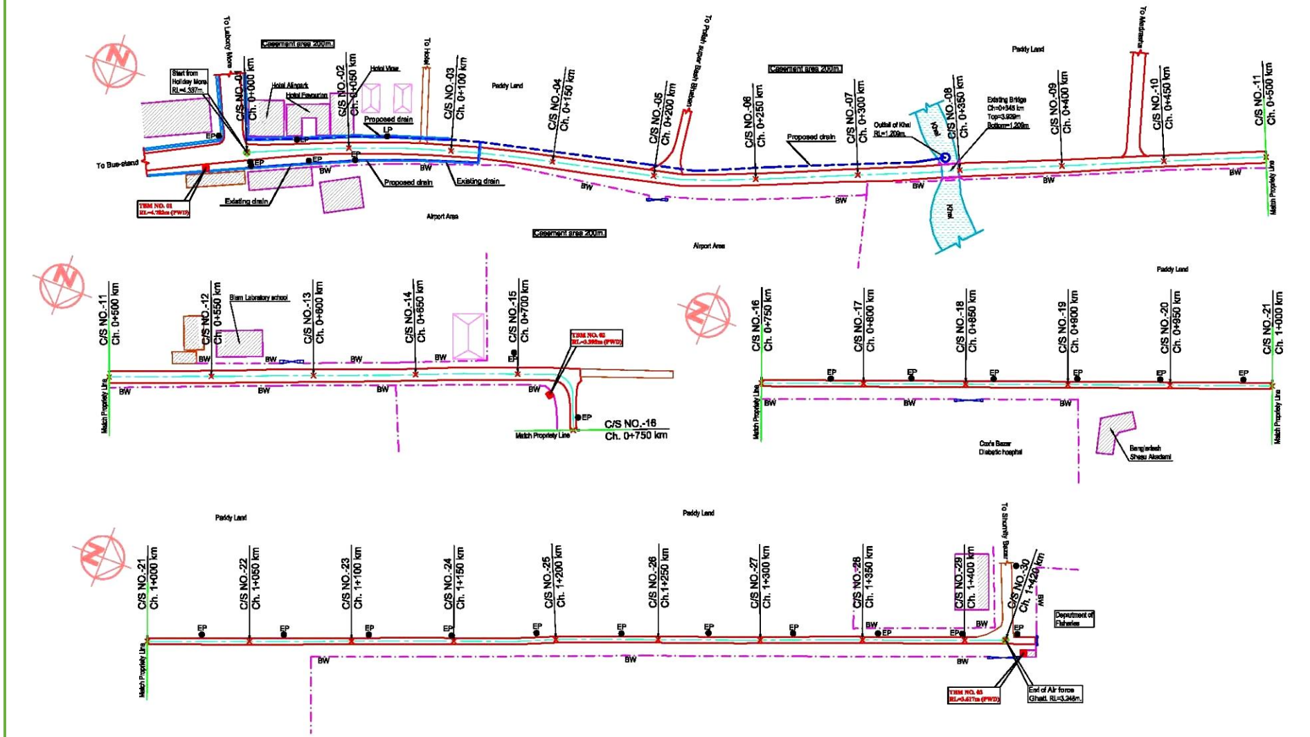
Figure 2.1.3 (a): Layout Plan for the proposed Subproject from Jeleepark to Air force Gate (1 st Part Road) at Cox's Bazar Pourashava
