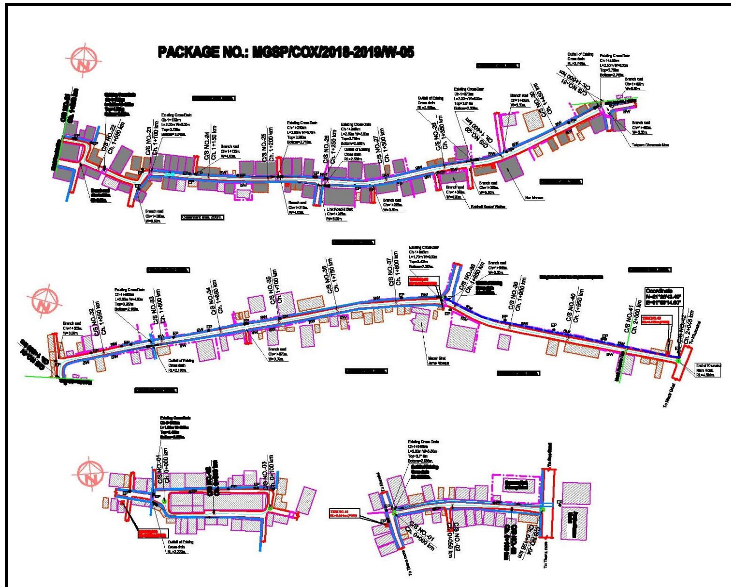
Figure 2.1.3 (b): Layout Plan for the proposed Subproject with Link Roads at Thana Road, Cox's Bazar Pourashava
