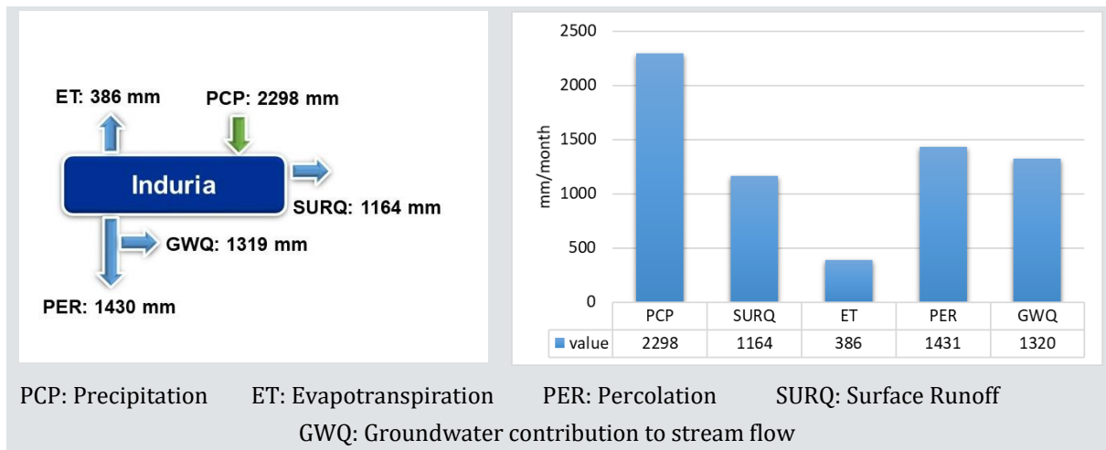
Figure 6.4: Average annual water balance (Induria village)
