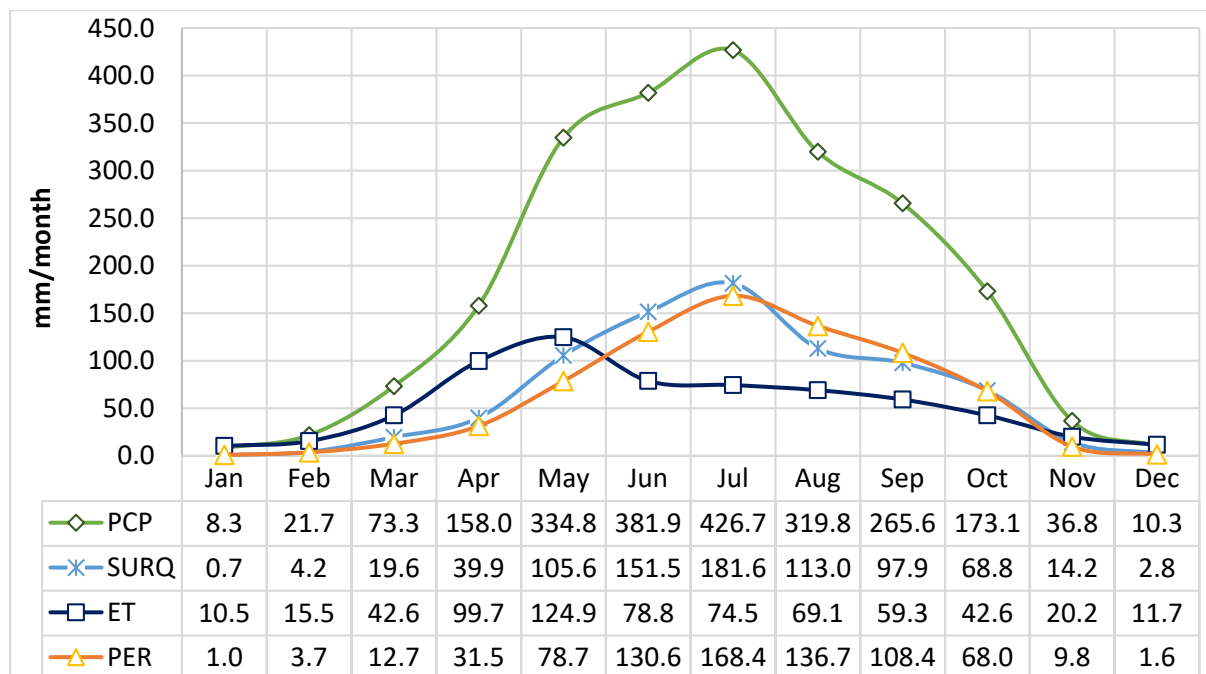
Figure 6.11: Average monthly water balance (Hafizpur village)
