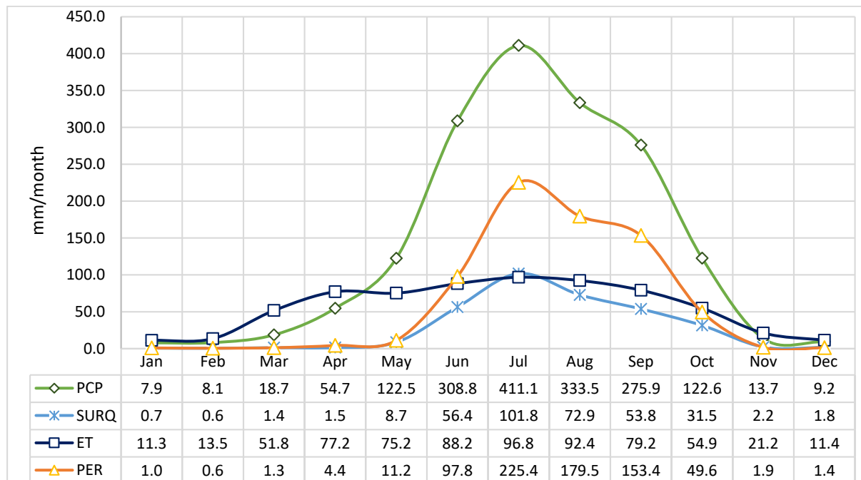
Figure 6.23: Average monthly water balance (Pathardabi village)
