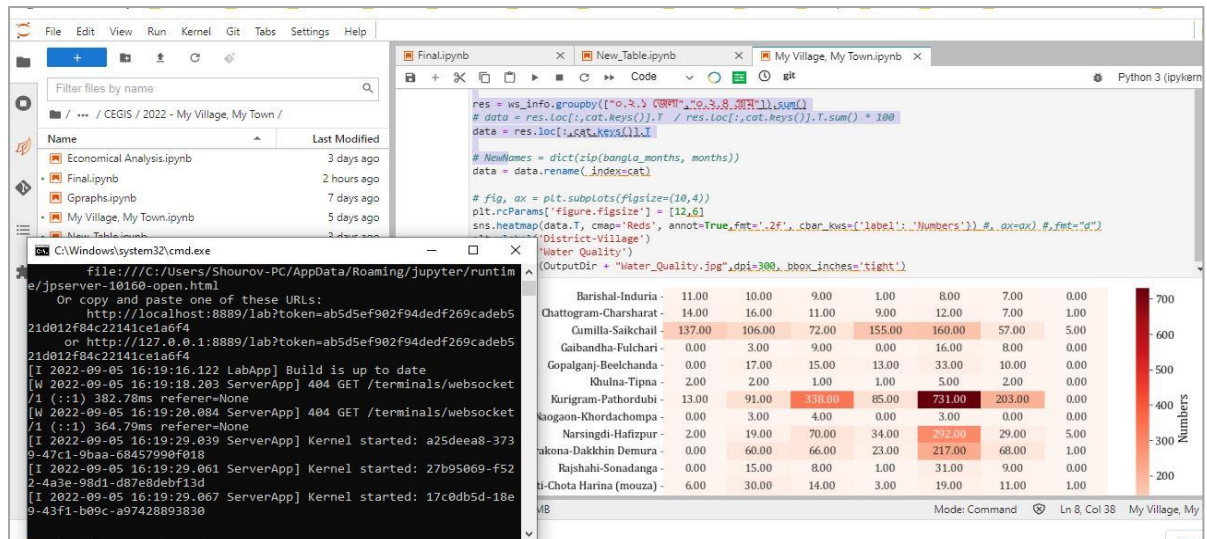
Figure I.6: Data analysis
