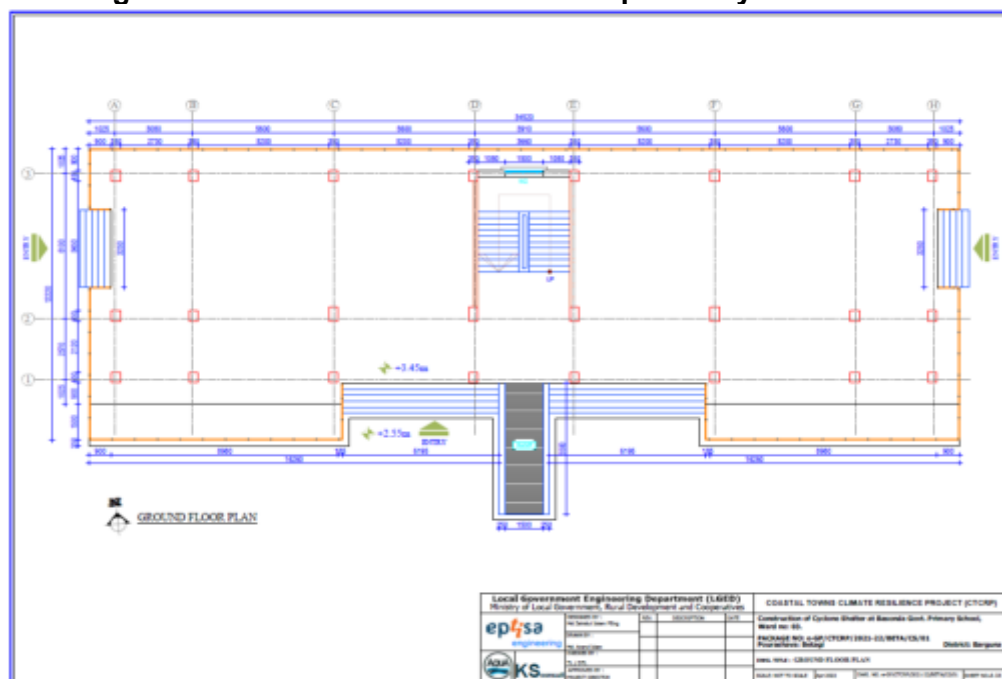
Figure 6: Ground Floor Plan of the Proposed Cyclone Shelter
