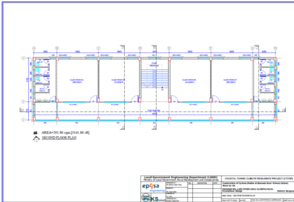
Figure 8: Second Floor Plan of the Proposed Cyclone Shelter
