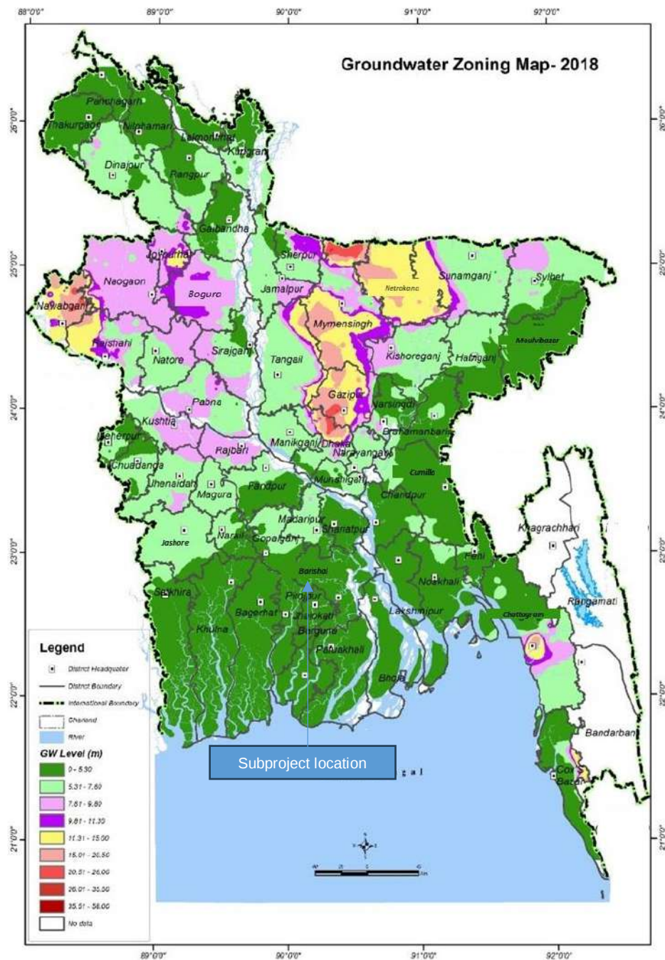
Figure 11: Ground Water Zoning Map
