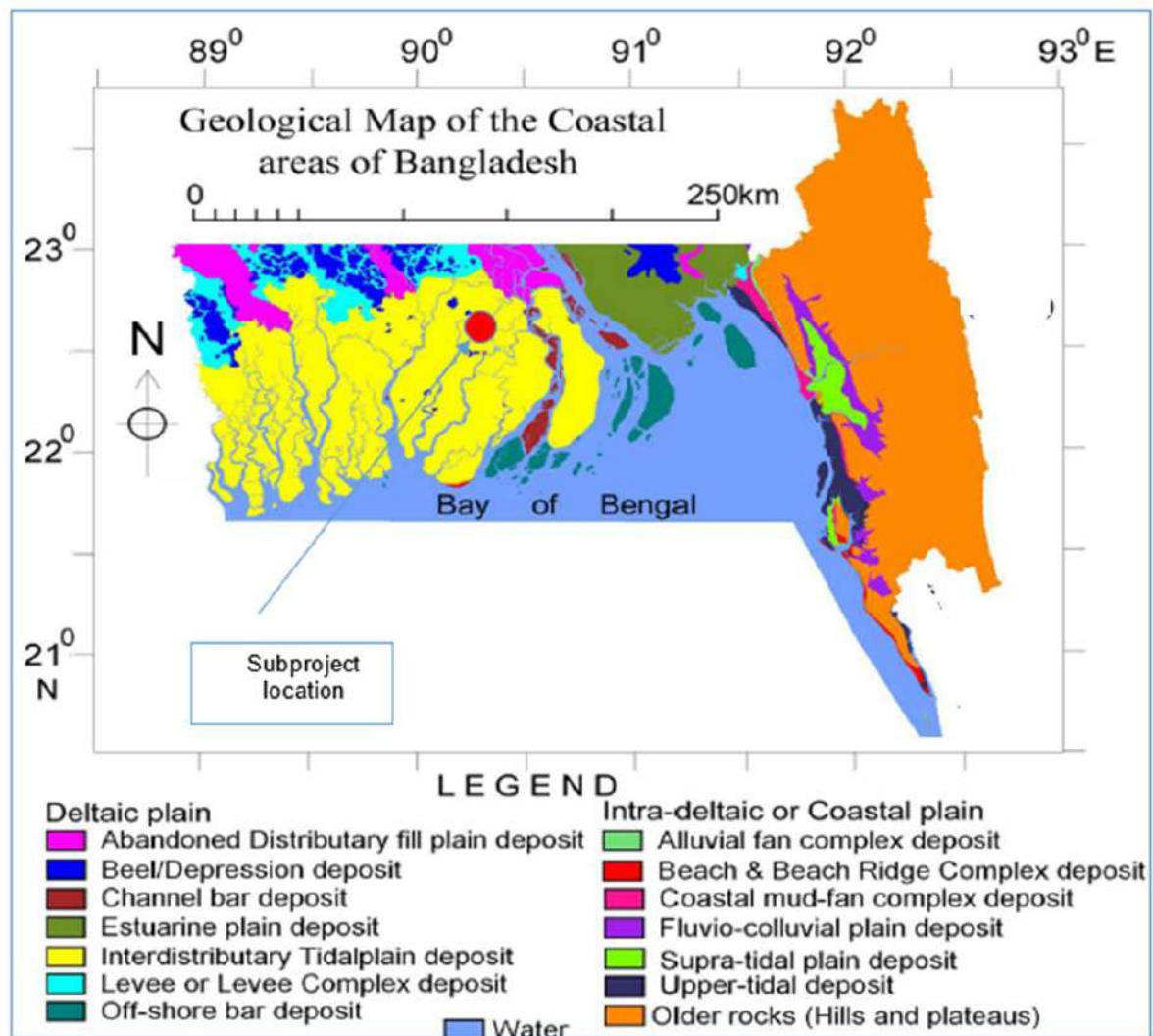
Figure 6: Geological Formation of Barishal Region
