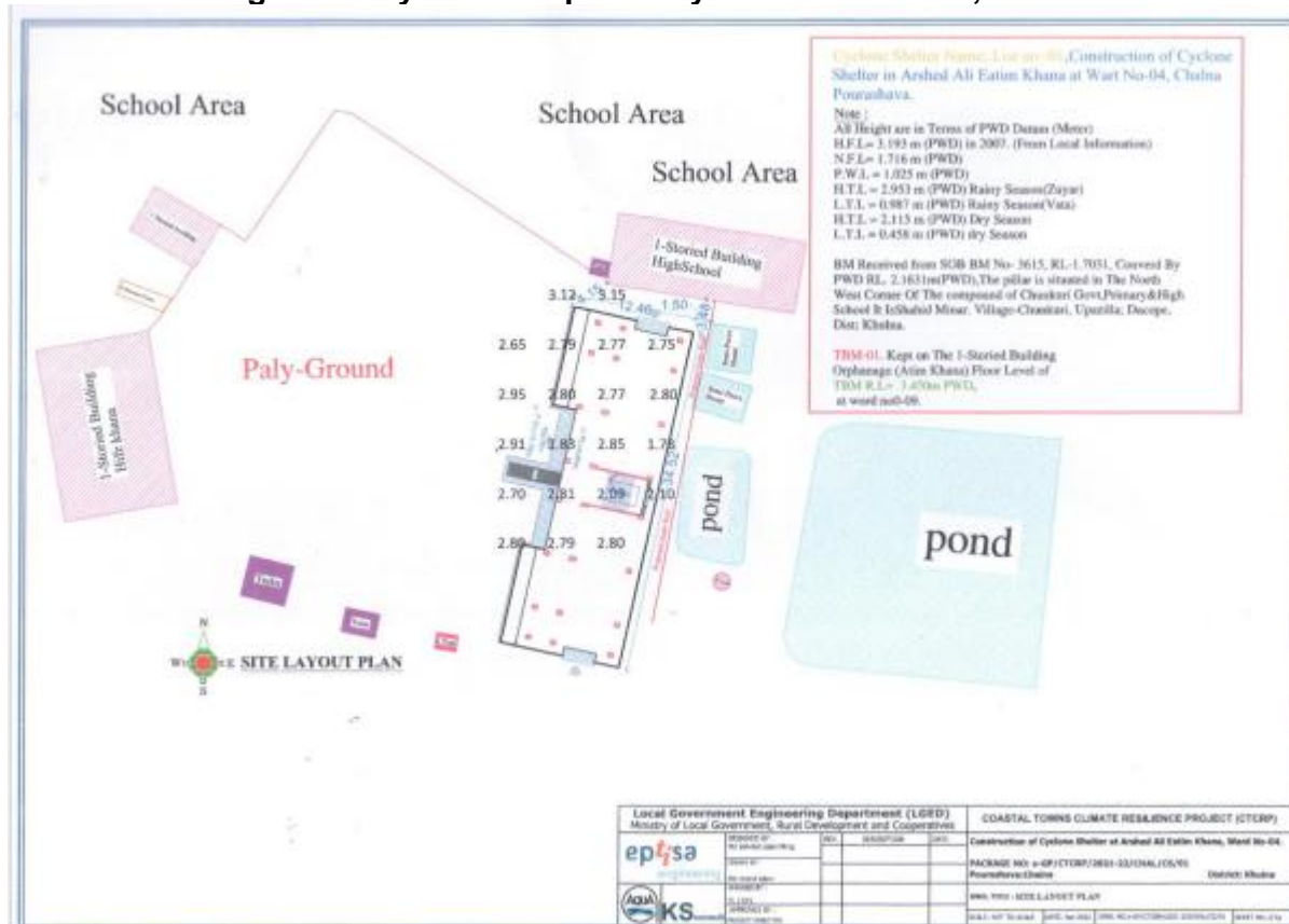
Figure 6: Layout of Proposed Cyclone Shelter Site, Chalna
