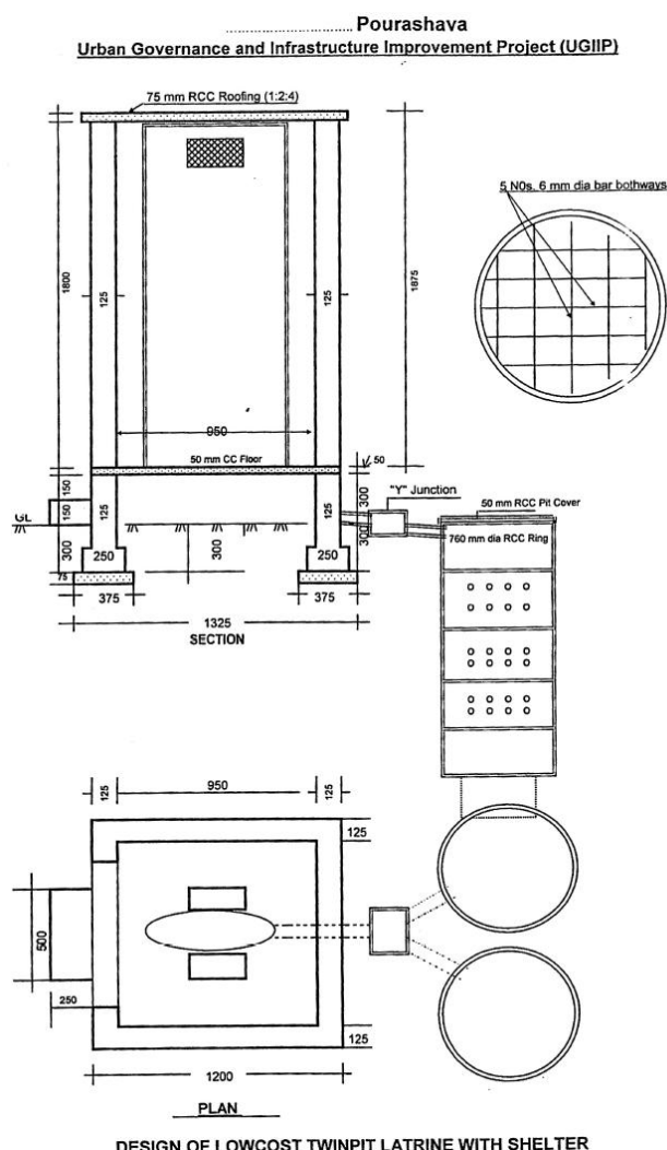
DESIGN OF LOWCOST TWINPIT LATRINE WITH SHELTER
