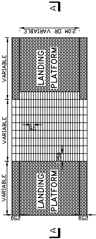
PLAN
