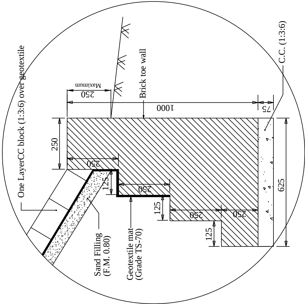
DETAIL-A PLATE UPR-UNR-EM2-2
