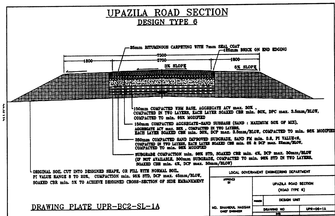
X-section: Design Type 6
