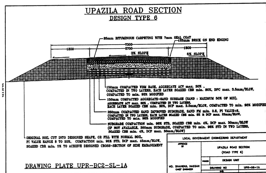
X-section: Design Type 6
