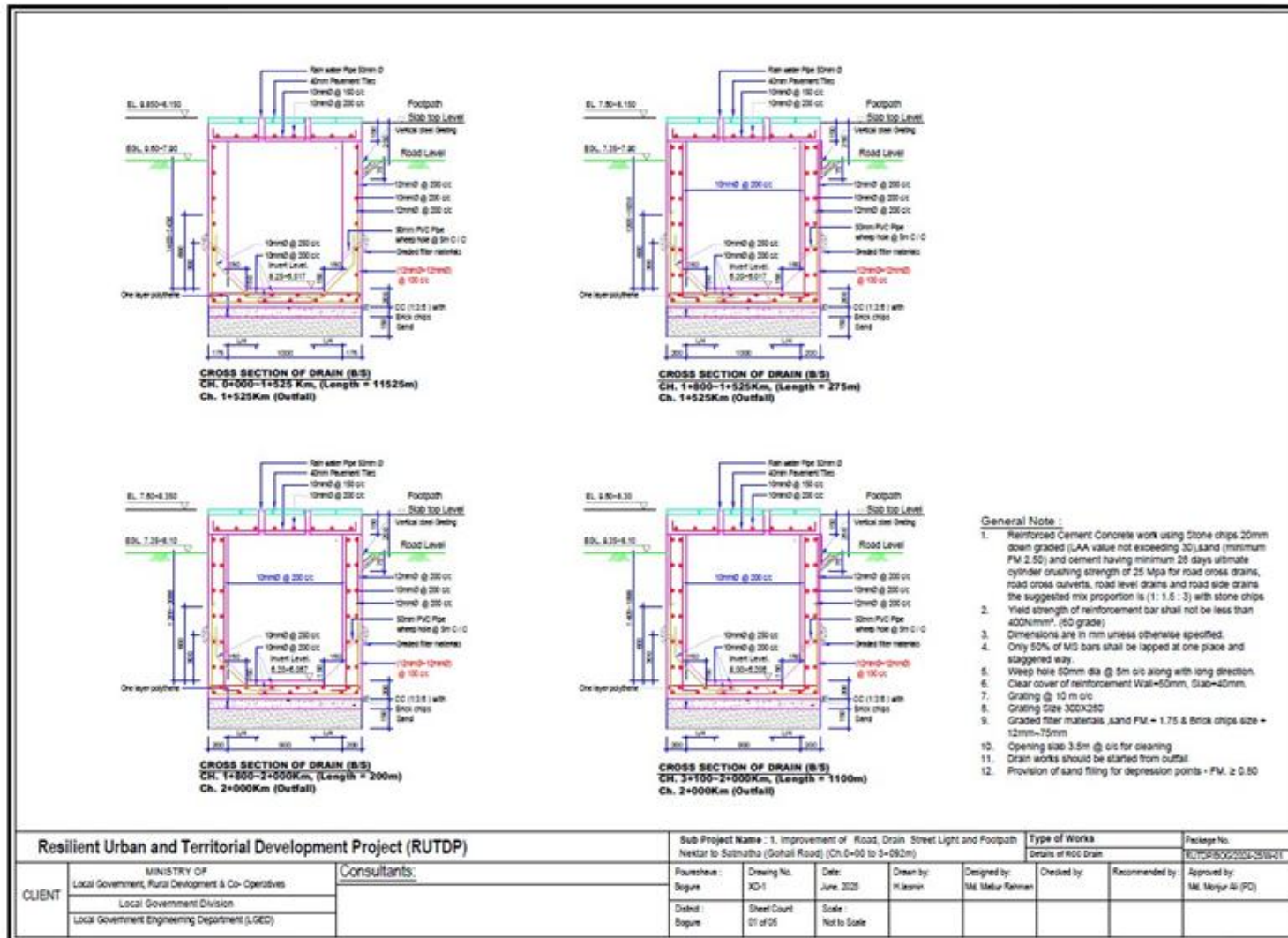
Figure 2.1.6: Cross-section of the Proposed Drainage Improvements
