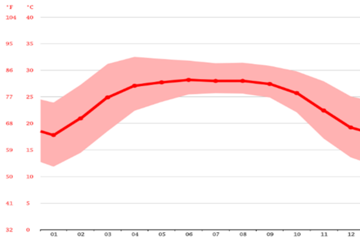
Figure 3.1.3: Climate Graph // Average Temperature by Month of Bogura Pourashava
