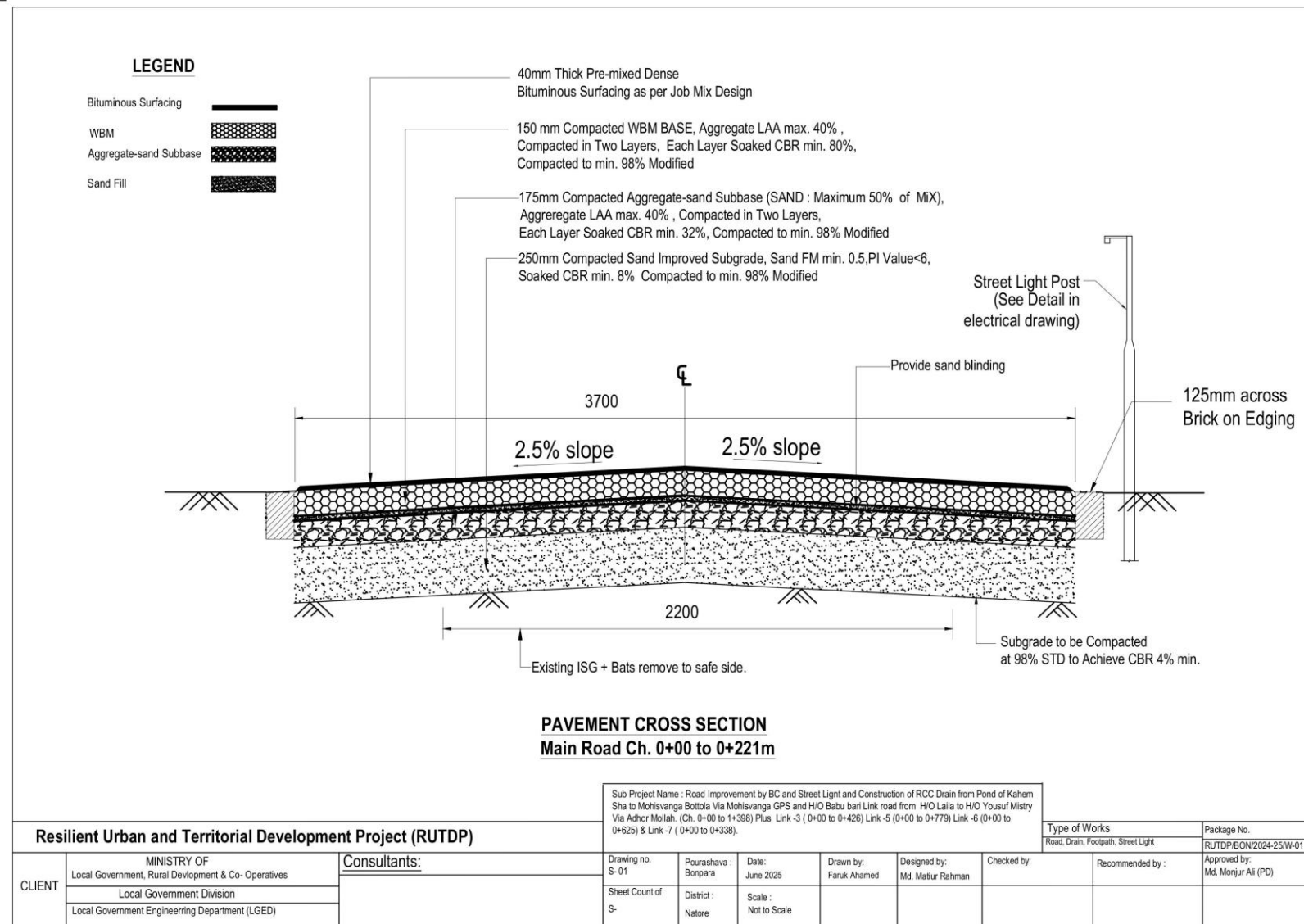
Figure 2.1.5: Cross-section of the Proposed BC Road Improvements
