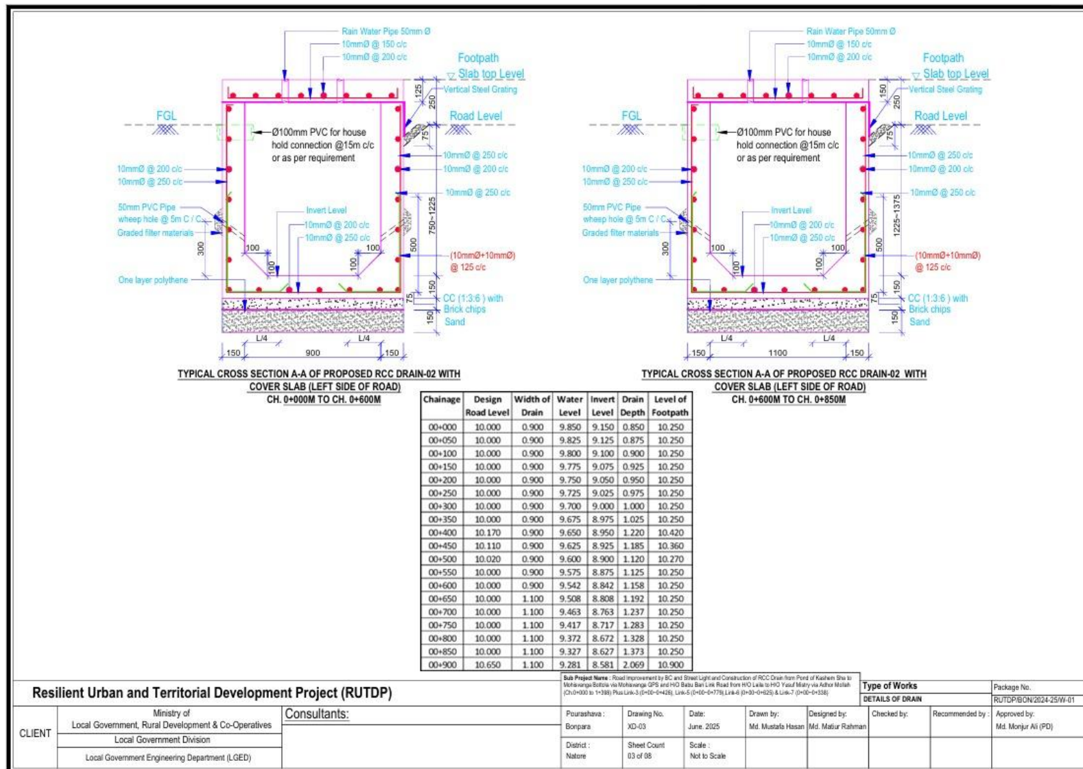
Figure 2.1.6: Cross-section of the Proposed Drainage Improvements
