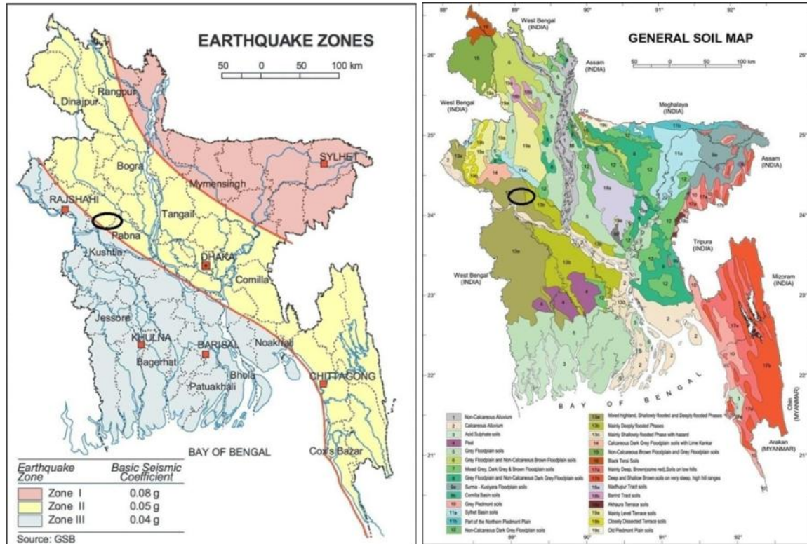
Figure 3.1.1: Location of Bonpara Pourashava in Earthquake Zoning map of Bangladesh [Source: BNBC,2006] and general soil map of Bangladesh [Source: BARC, 2005] (the Black circle denotes Bonpara Pourashava)
