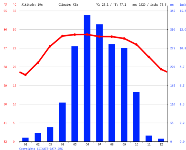
Figure 3.1.2: Climate Graph // Weather by Month of Bonpara Pourashava
