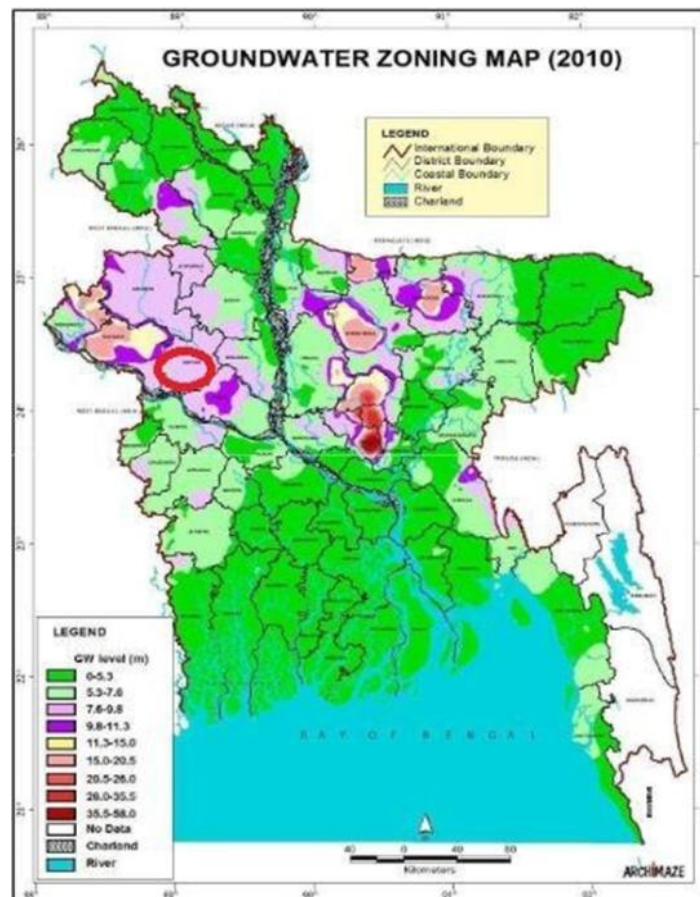
Figure 3.1.4: Location of Bonpara Pourashava in Groundwater Zoning Map of Bangladesh [Source: BADC, 2010] (the red circle denotes Bonpara Pourashava)
