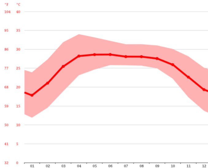
Figure 3.1.3: Climate Graph // Average Temperature by Month of Bonpara Pourashava
