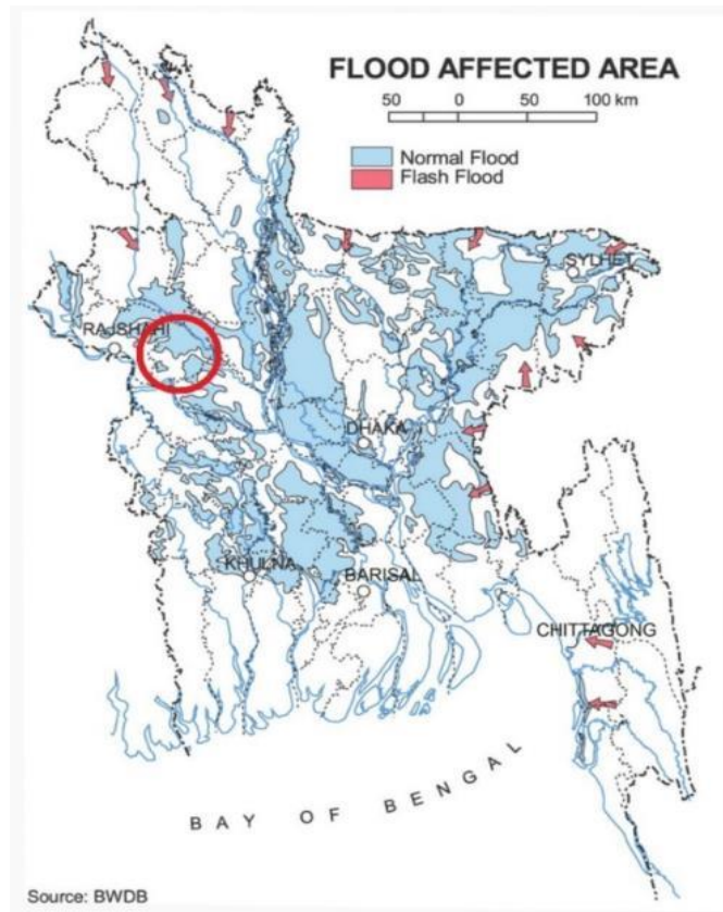
Figure 3.1.5: Location of Bonpara Pourashava in Flood Zone Map of Bangladesh [Source: BMD]
