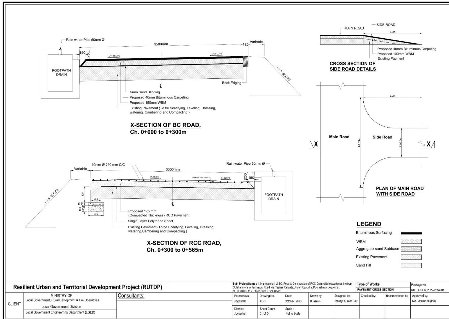
Figure 2.1.6: Cross-section, of the proposed BC and RCC road for the Pourashava
