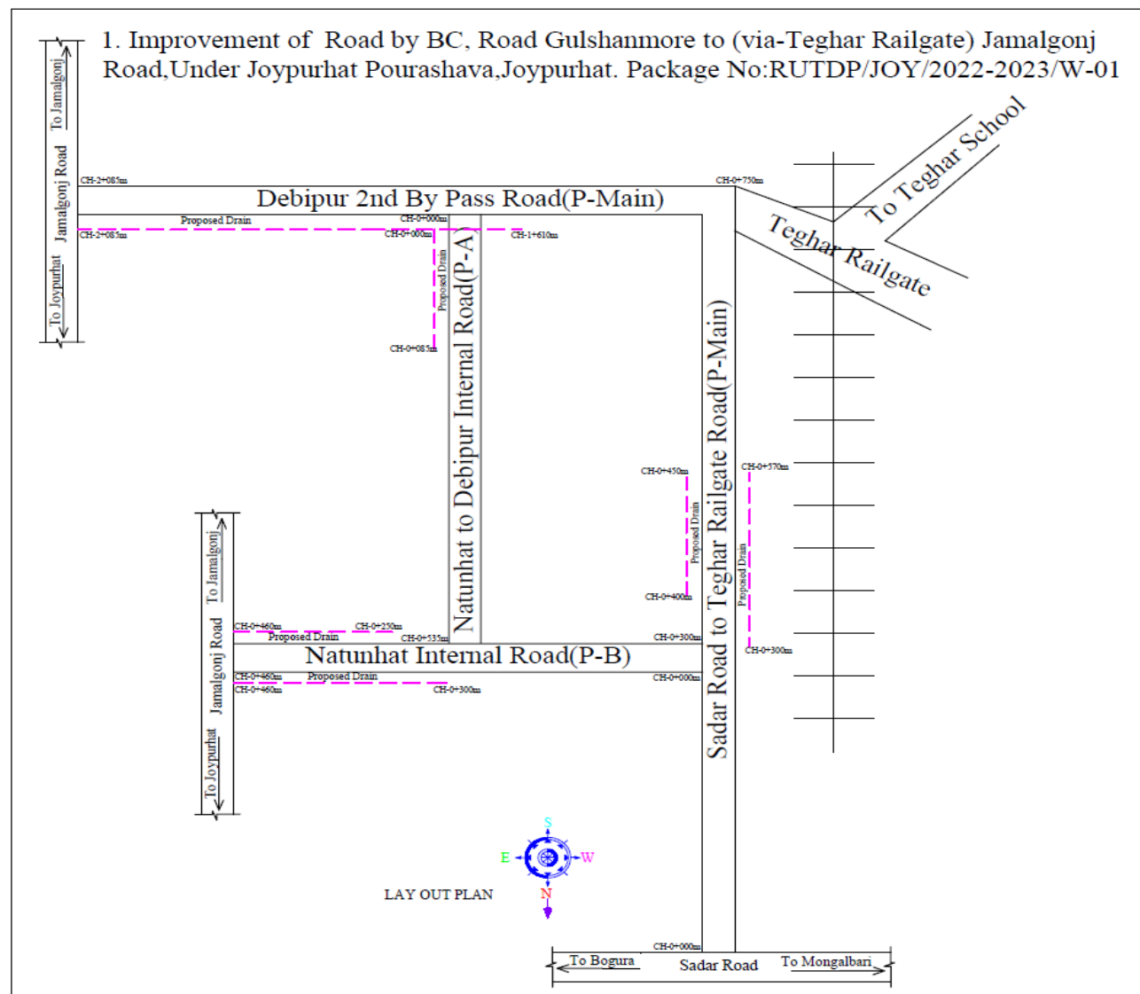
Figure 2.1.4: Zone Layout Plan of the Proposed Subproject Area from Gulshanmore to Jamalgonj road via Teghar Railgate
