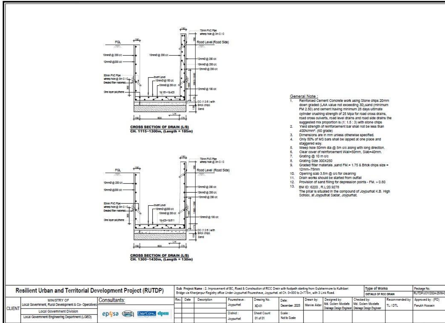
Figure 2.1.7: Cross-section of the Proposed Drainage Improvements
