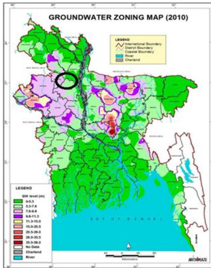
Figure 3.1.4: Location of Singra Pourashava in Groundwater Zoning Map of Bangladesh [Source: BADC, 2010] (the black circle denotes Singra Pourashava)
