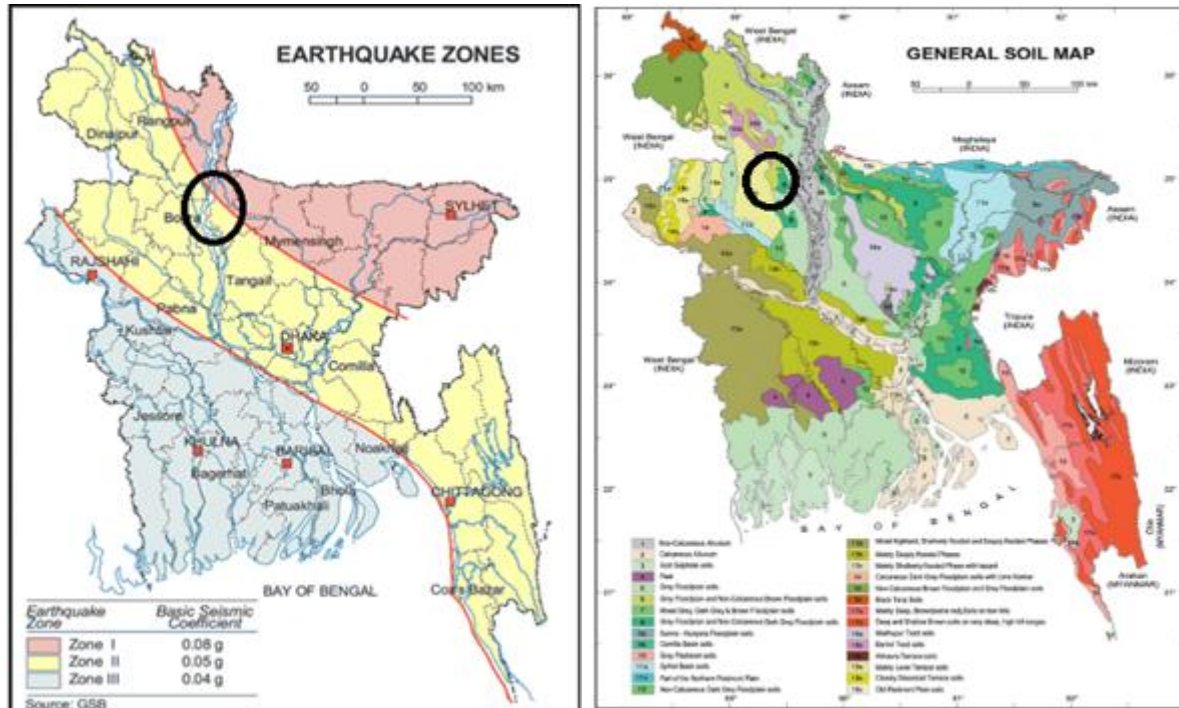
Figure 3.1.1: Location of Singra Pourashava in Earthquake Zoning map of Bangladesh [Source: BNBC,2006] and general soil map of Bangladesh [Source: BARC, 2005] (the Black circle denotes Singra Pourashava)
