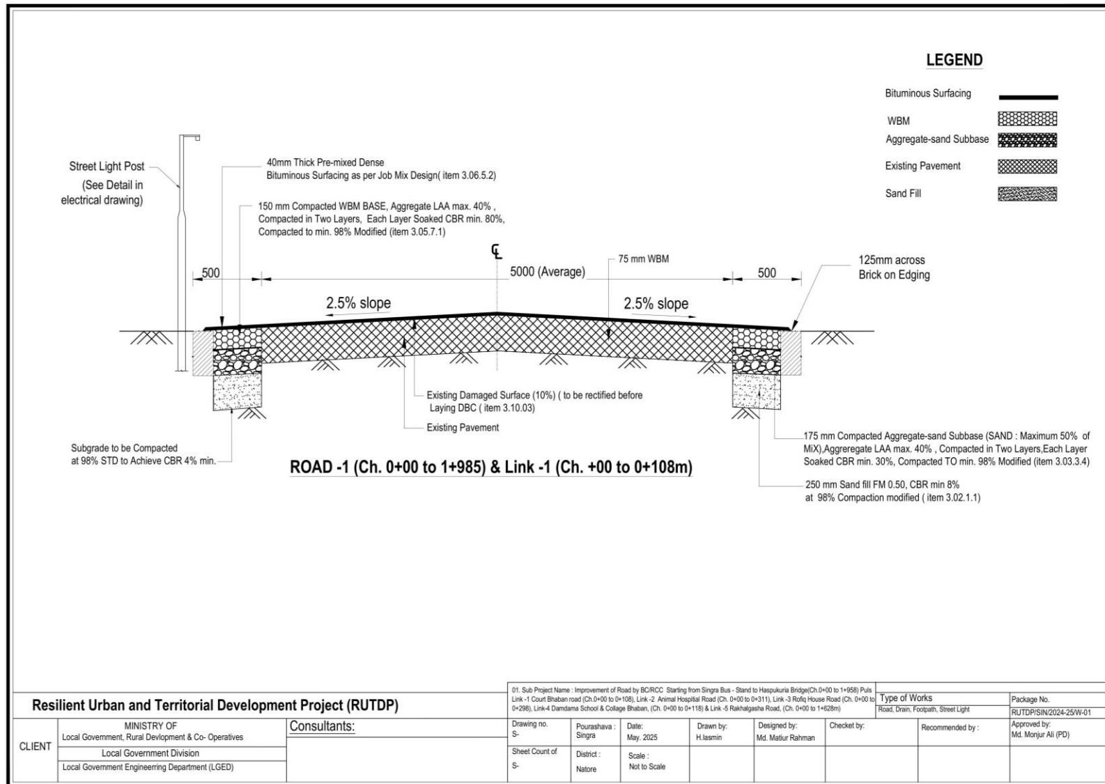
Figure 2.1.5: Cross-section, of the proposed BC and RCC road for the Pourashava
