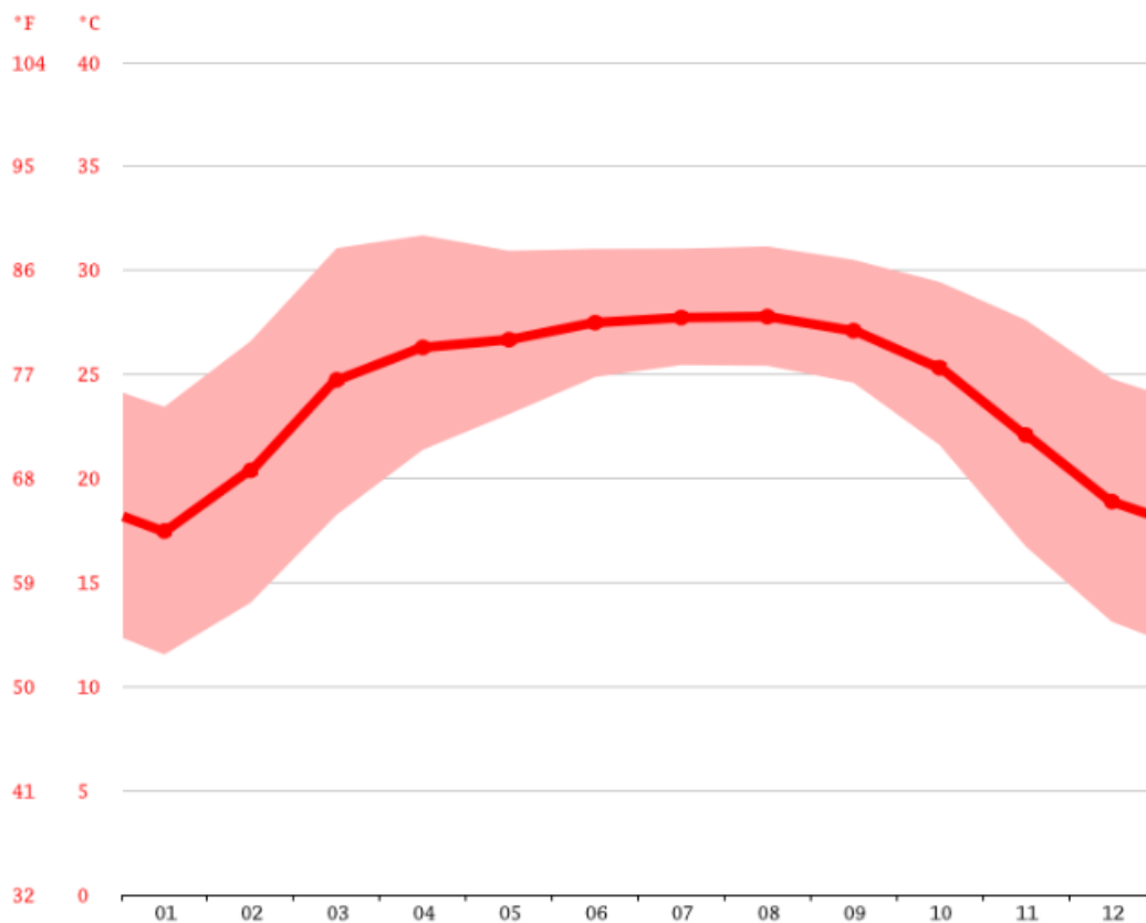
Figure 3.1.3: Climate Graph // Average Temperature by Month of Saidpur Pourashava
