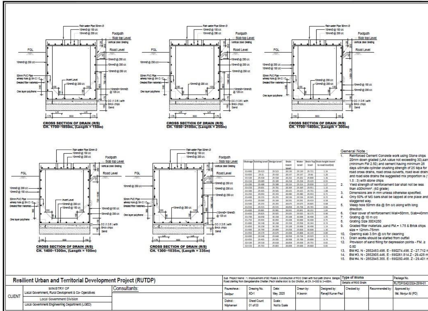
Figure 2.1.7: Cross-section of the Proposed Drainage Improvement
