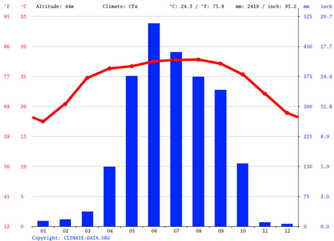
Figure 3.1.2: Climate Graph // Weather by Month of Saidpur Pourashava
