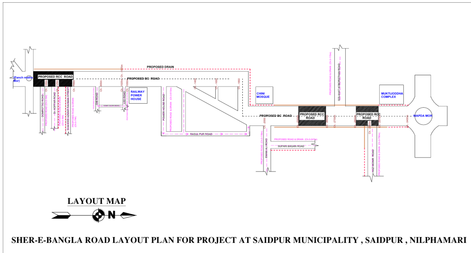
Figure 2.1.5: Layout Plan of the Proposed Subproject Area (Road) and its Adjoining Roads with Influence Zone
