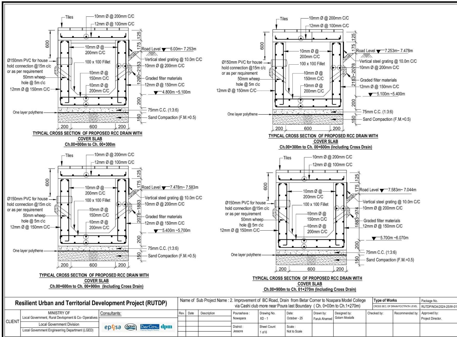
Figure 2.1.7: Cross-section of the Proposed Drainage Improvements
