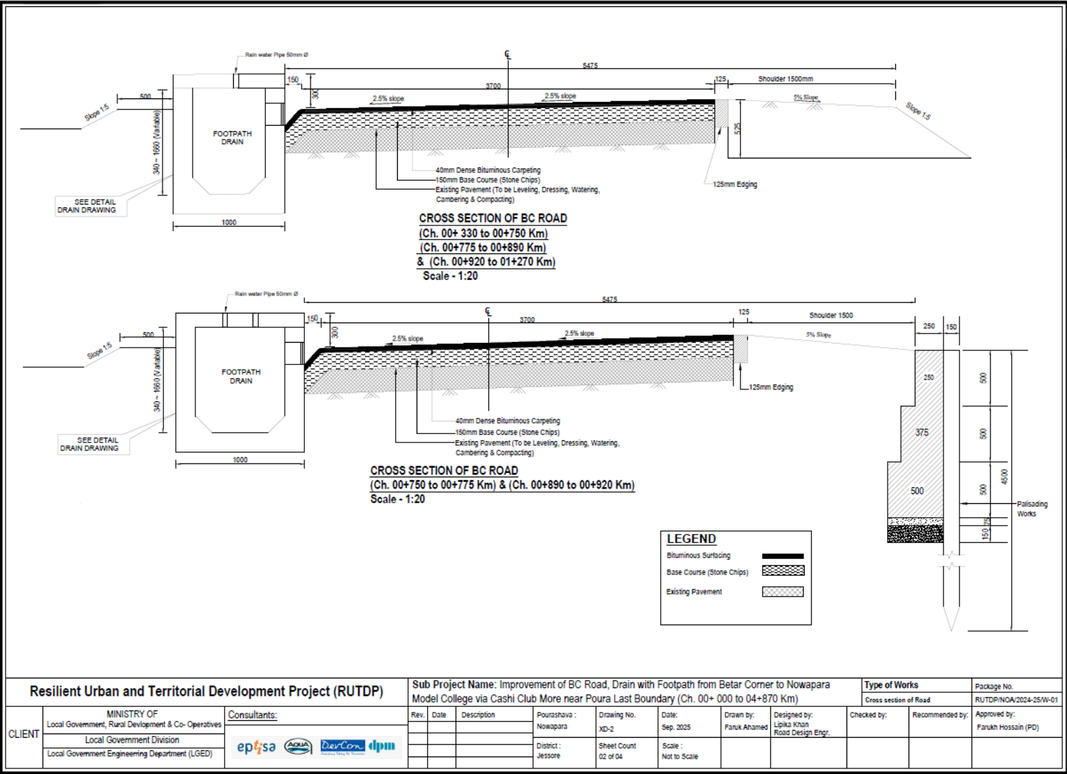
Figure 2.1.6: Cross-section of the Proposed BC Road Improvements
