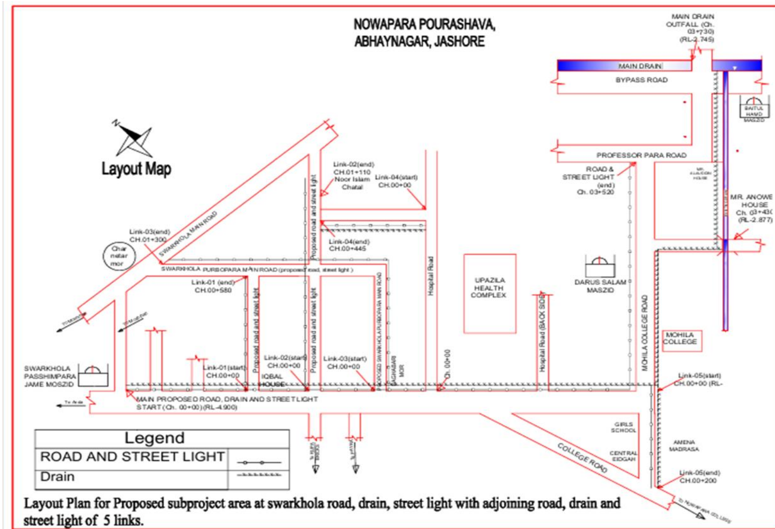
Figure 2.1.4: Zone Layout Plan of the Proposed Subproject Area (Road) and its Adjoining Roads with Influence Zone
