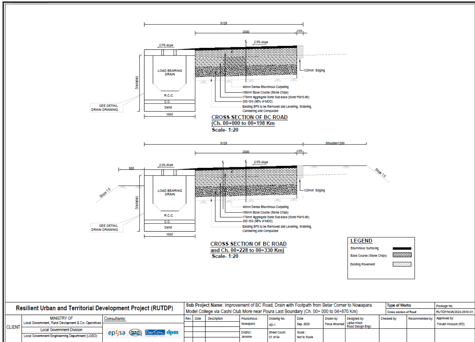
Figure 2.1.5: Cross-section of the Proposed BC Road Improvements
