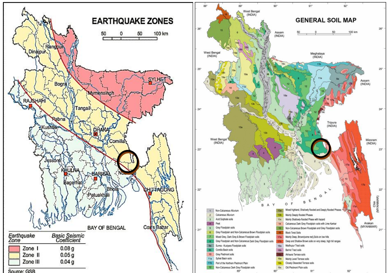
Figure 3.1.1: Location of Feni Pourashava in Earthquake Zoning map of Bangladesh [Source: GSB, 1978] and general soil map of Bangladesh [Source: BARC, 2005] (the black circle denotes Feni Pourashava)
