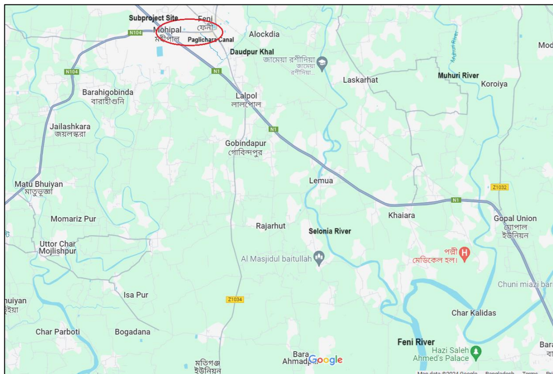
Figure 3.1.4: Natural drainage pattern of Feni Pourashava [Source: Google map]
