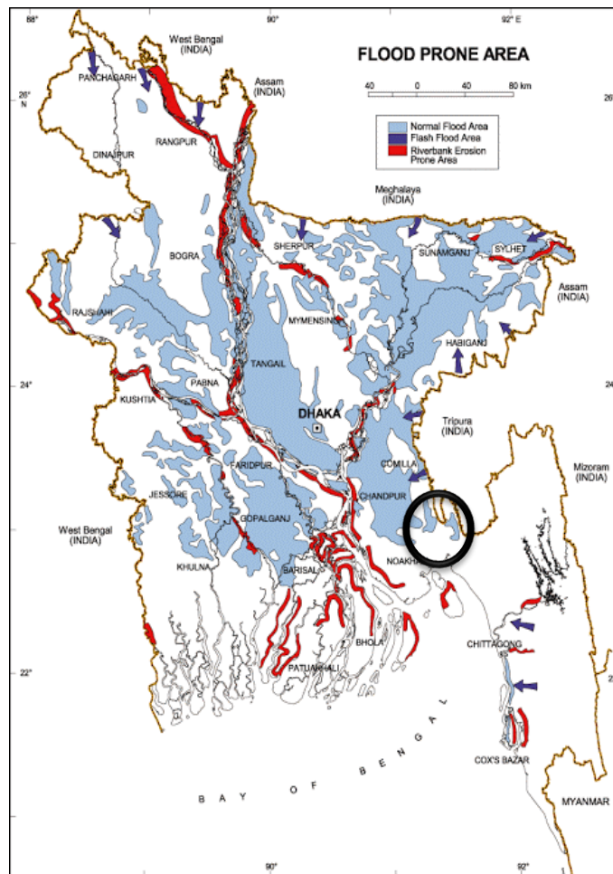
Figure 3.1.3: Location of Feni Pourashava in Flood Zone Map of Bangladesh [Source: BMD]
