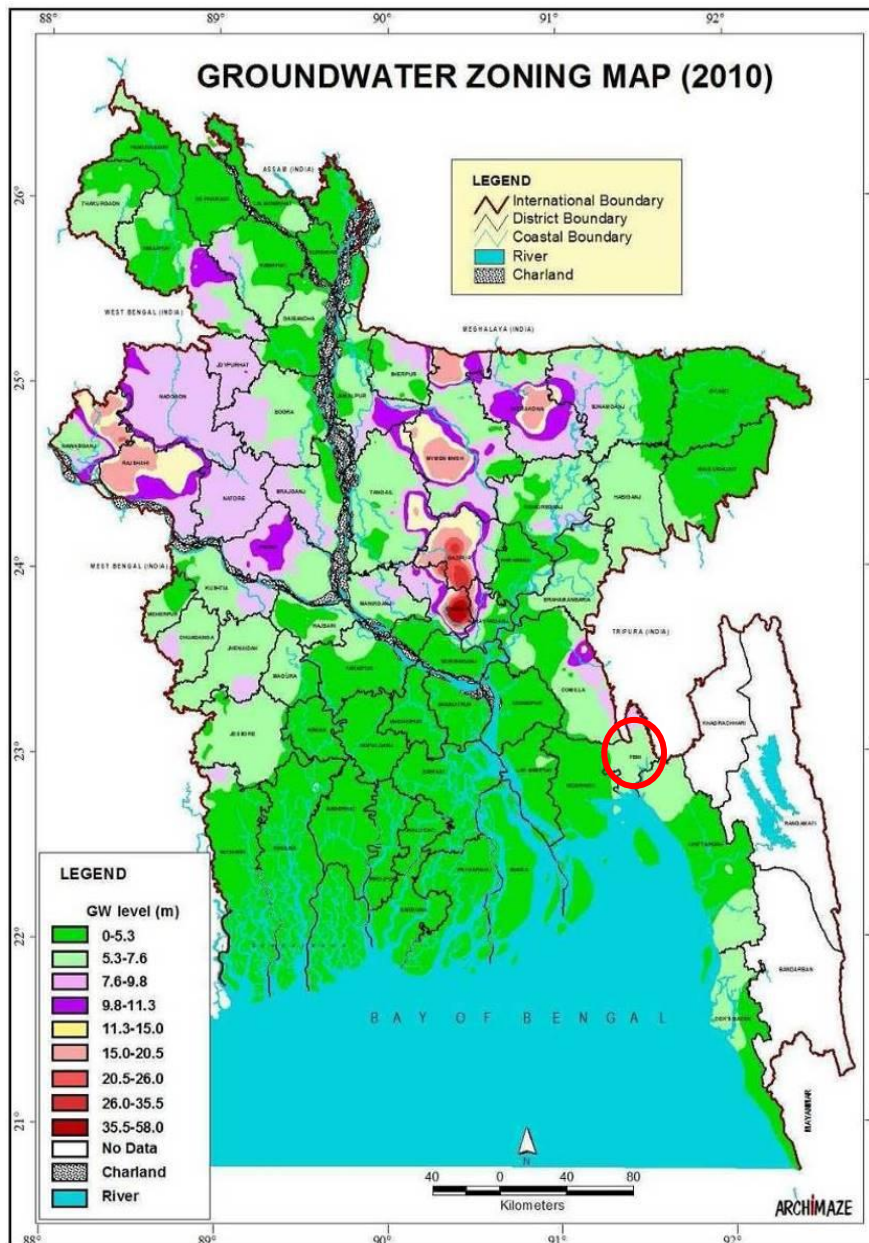
Figure 3.1.2: Location of Feni Pourashava in Groundwater Zoning Map of Bangladesh [Source: BADC, 2010] (the red circle denotes Feni Pourashava)
