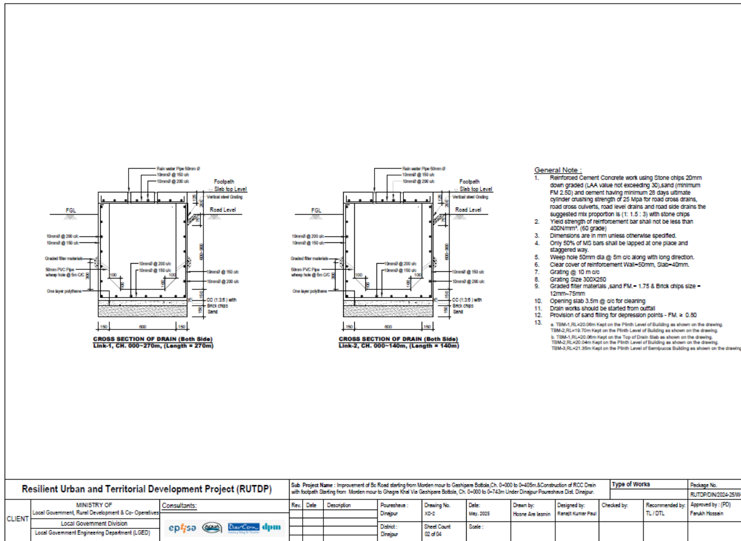
Figure 2.1.9: Cross-section of the Proposed Drainage Improvement
