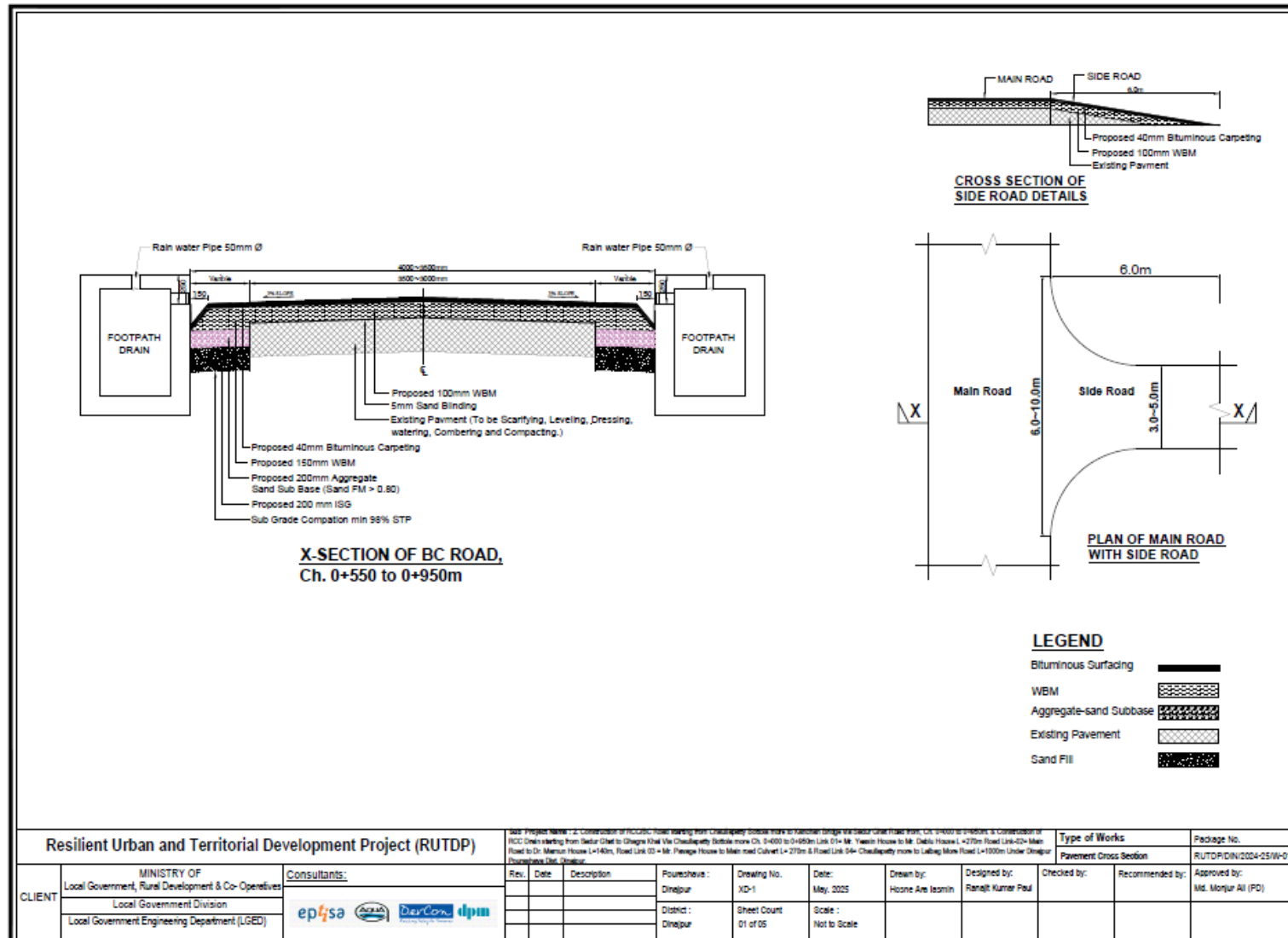
Figure 2.1.8: Cross-section of the proposed BC Road Improvements for the Pourashava
