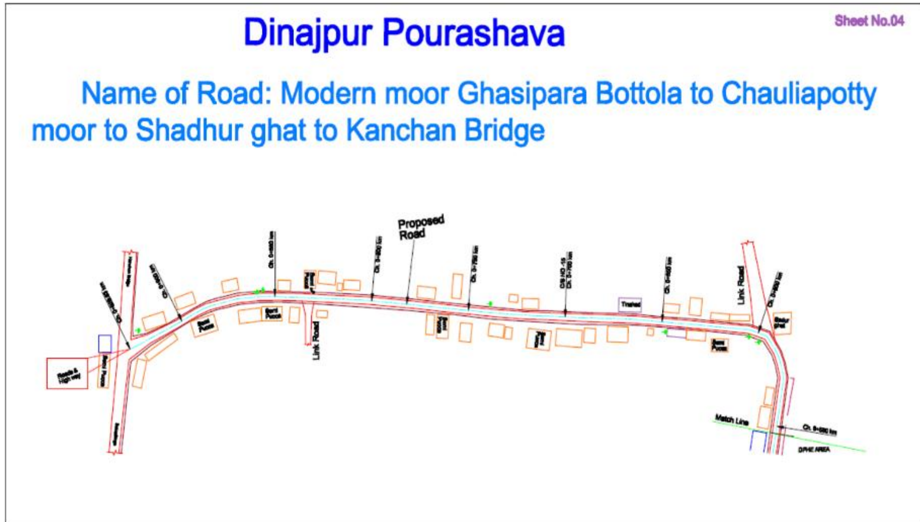
Figure 2.1.6: Layout Plan of the Proposed Subproject Area and its Adjoining Roads with Influence Zone
