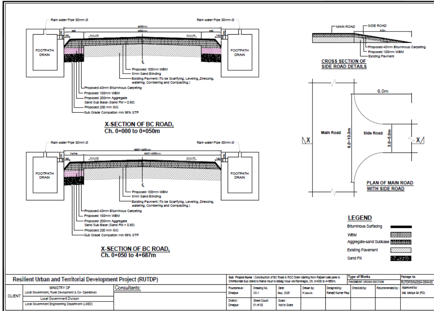
Figure 2.1.9: Cross-section of the proposed BC Road Improvements for the Pourashava
