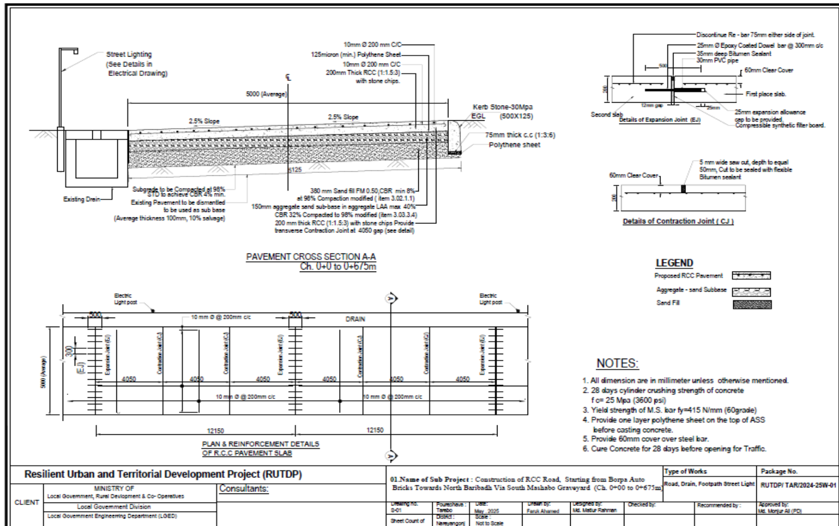
Figure 2.1.5: Cross-section of the proposed RCC Road Improvements for the Pourashava
