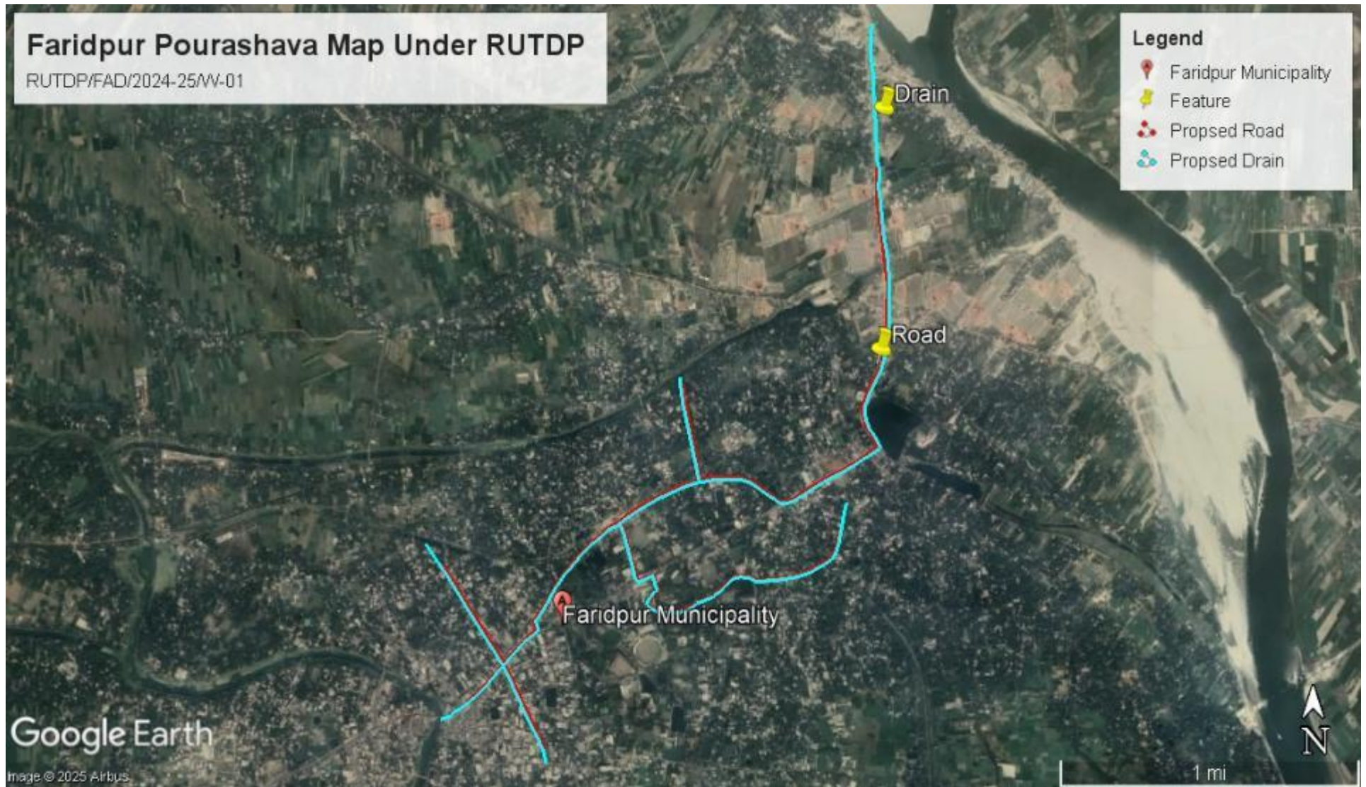
Figure 2.1.1 Topographic Features of the Subproject Area and its Adjoining Roads with Influence Zone
