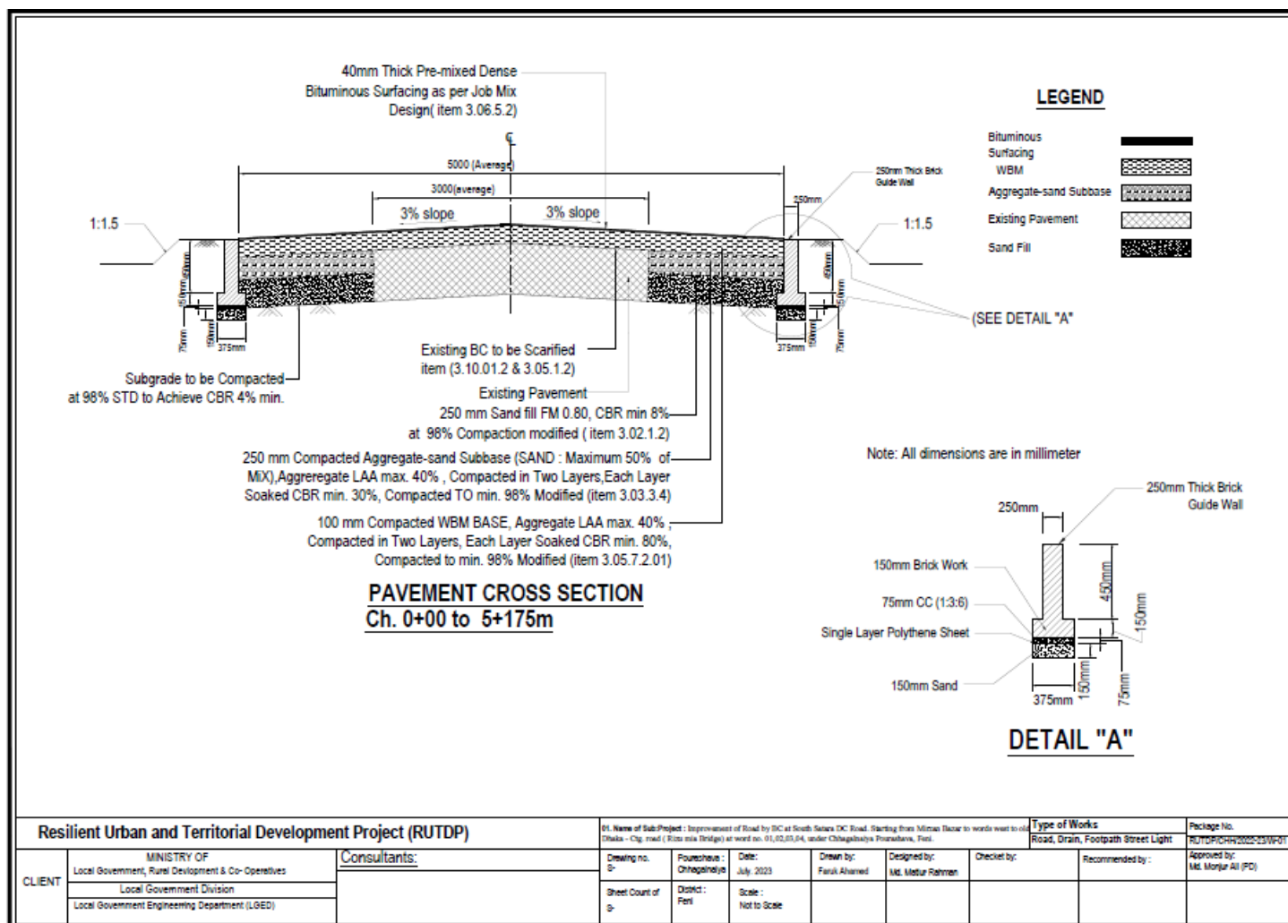
Figure 2.1.5: Cross-section of BC Road of the subproject
