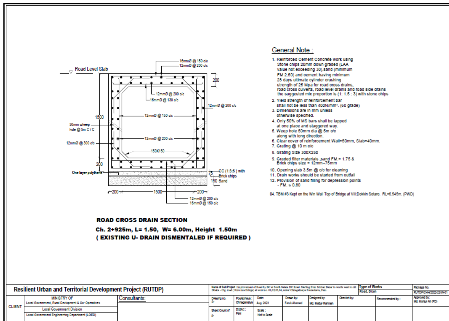
Figure 2.1.4: Cross-section of RCC Drain of the subproject
