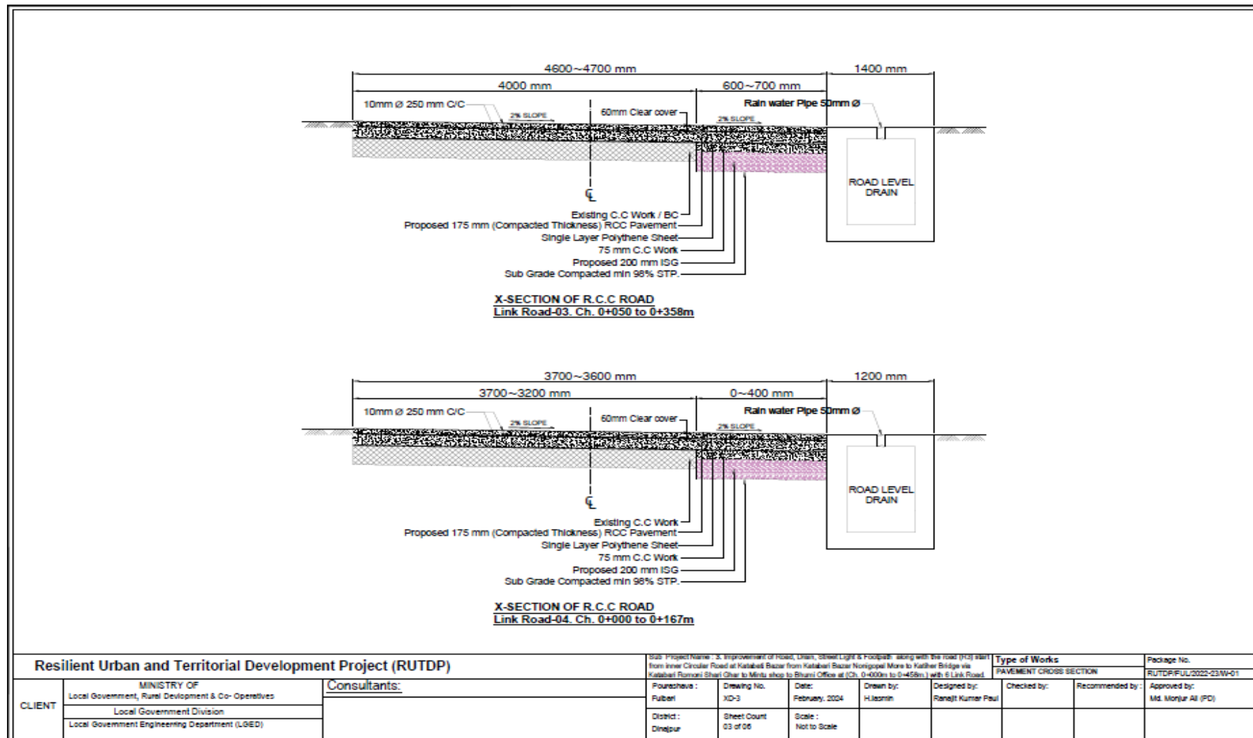
Figure 2.1.6: Cross-section of the proposed BC Road Improvements for the Pourashava
