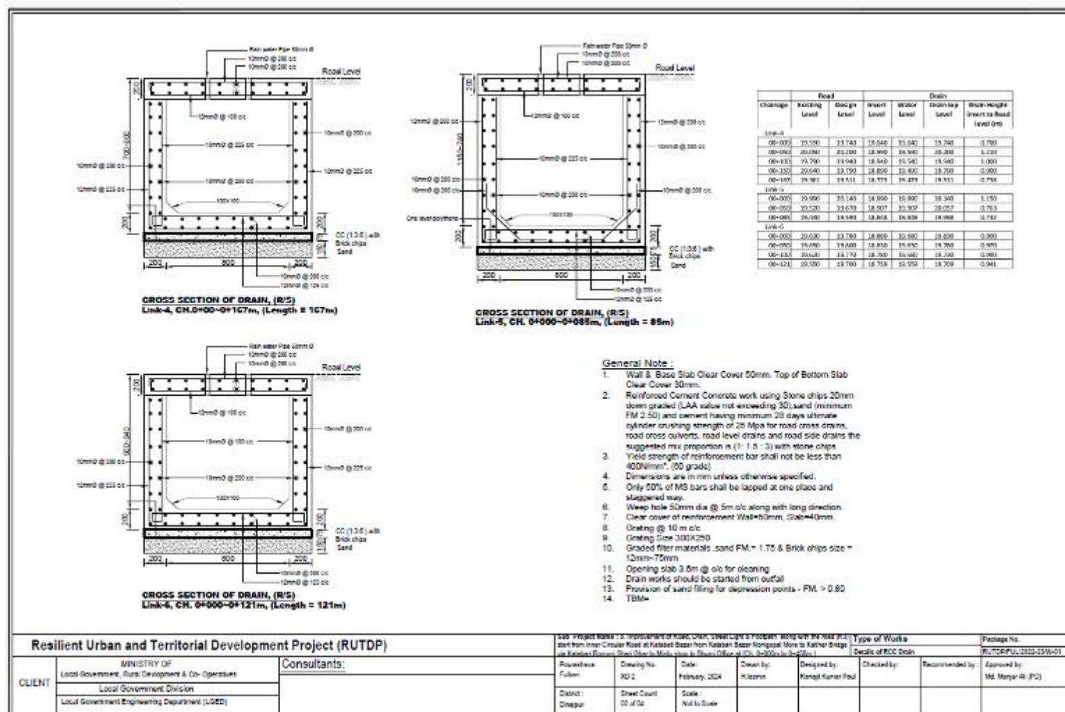
Figure 2.1.7: Cross-section of the Proposed Drainage Improvement
