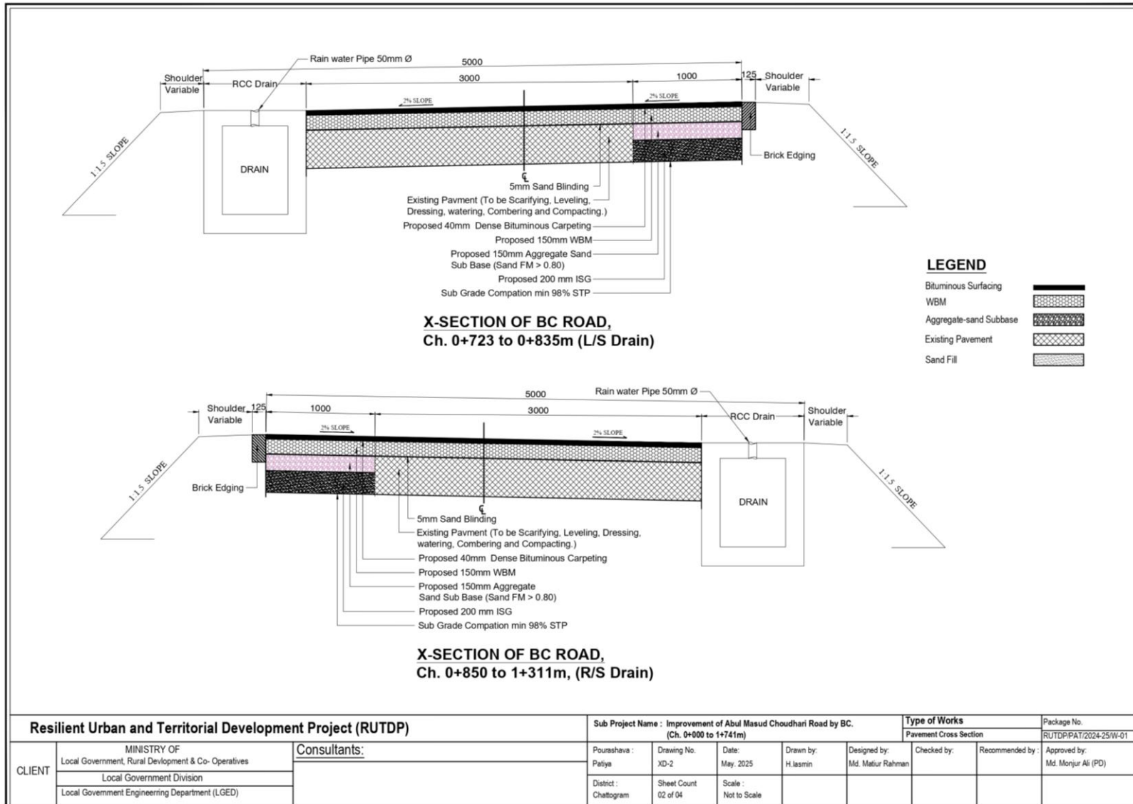
Figure 2.1.6: Cross-section of the proposed RCC Road Improvements for the Pourashava
