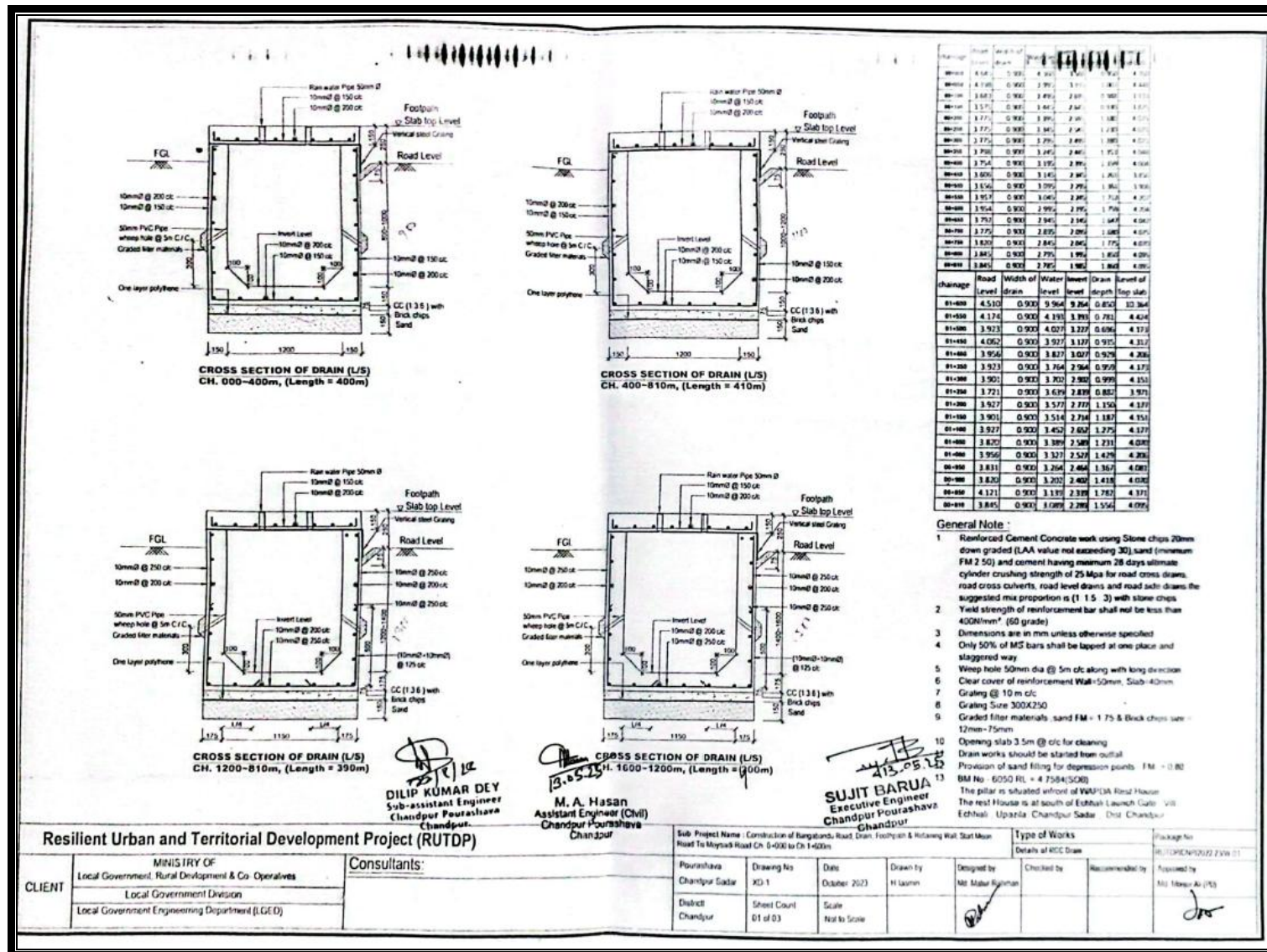
Figure 2.1.5: Cross-section of the RCC Drain of the proposed subproject area
