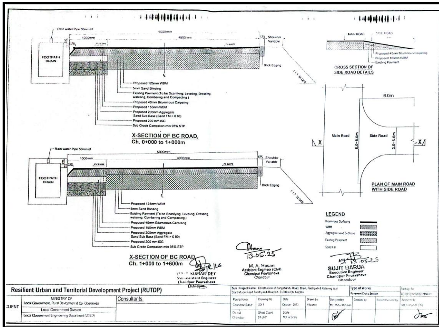
Figure 2.1.4: Cross-section of the BC Road of the proposed subproject area
