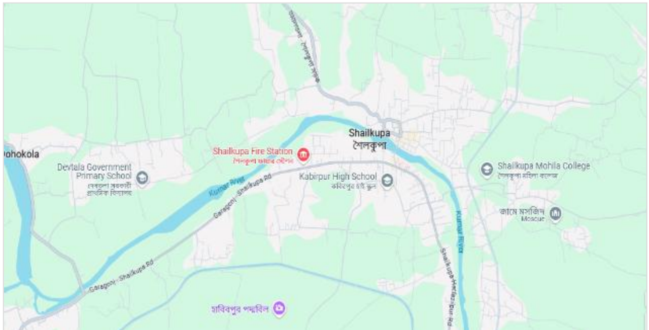
Figure 3.1.4: Natural drainage pattern of Shaikupa Pourashava [Source: Google map]
