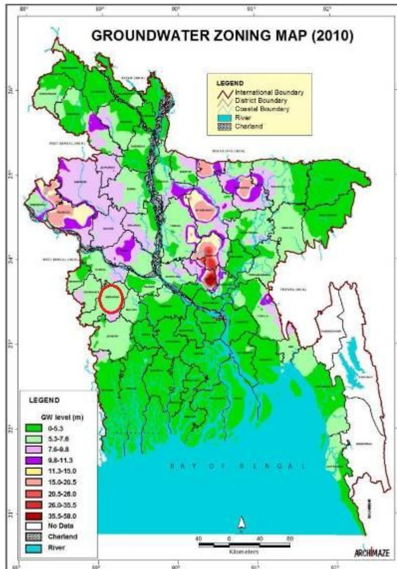
Figure 3.1.2: Location of Shaikupa Pourashava in Groundwater Zoning Map of Bangladesh [Source: BADC, 2010] (the red circle denotes Shaikupa Pourashava)
