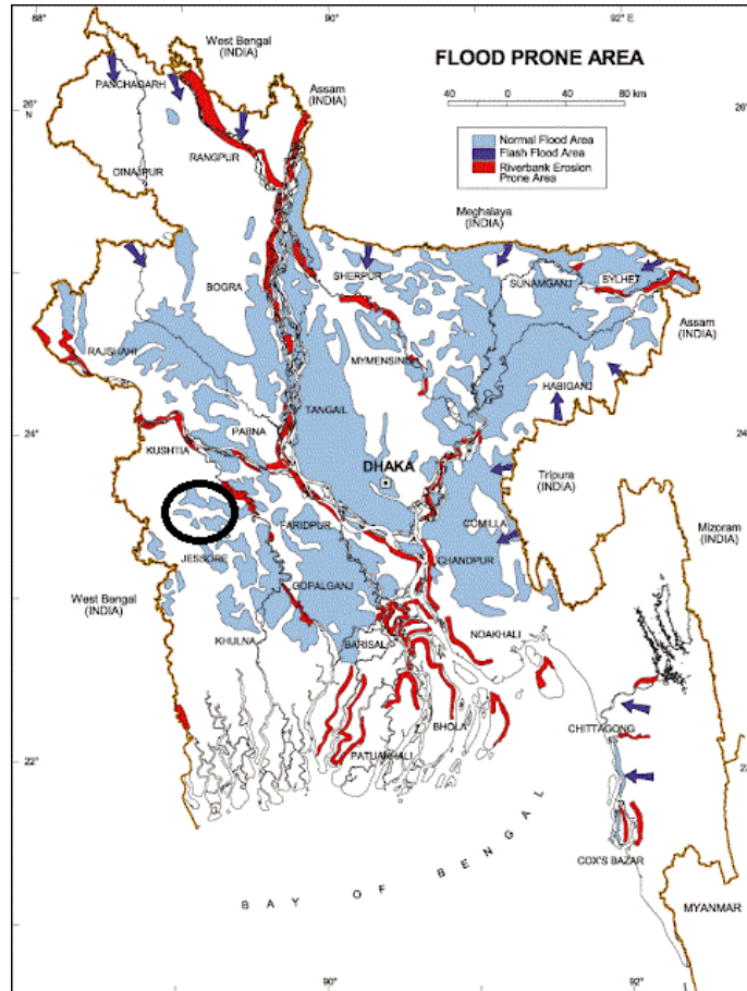
Figure 3.1.3: Location of Shaikupa Pourashava in Flood Zone Map of Bangladesh [Source: BMD]
