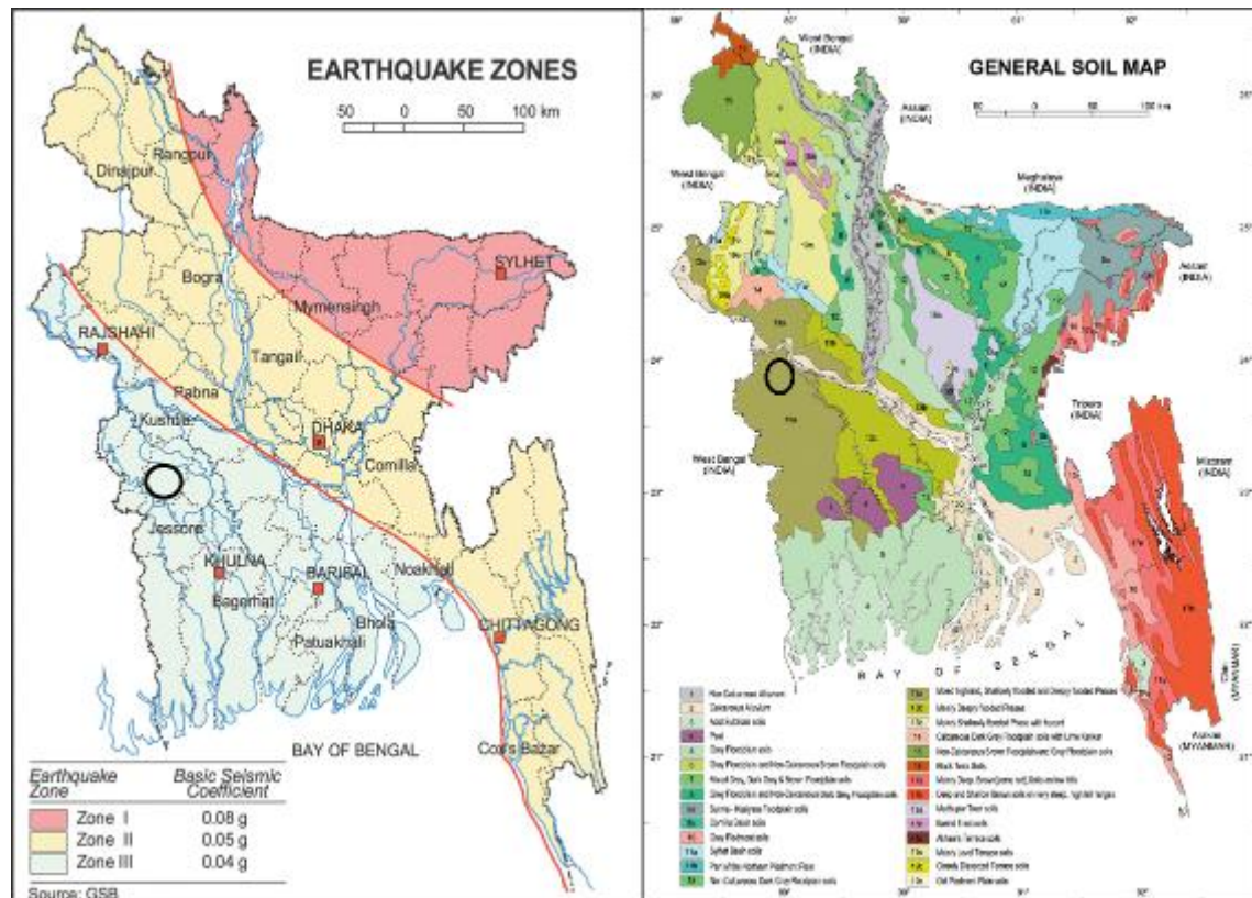
Figure 3.1.1: Location of Shaikupa Pourashava in Earthquake Zoning map of Bangladesh [Source: GSB, 1978] and general soil map of Bangladesh [Source: BARC, 2005] (the black circle denotes Shaikupa Pourashava)
