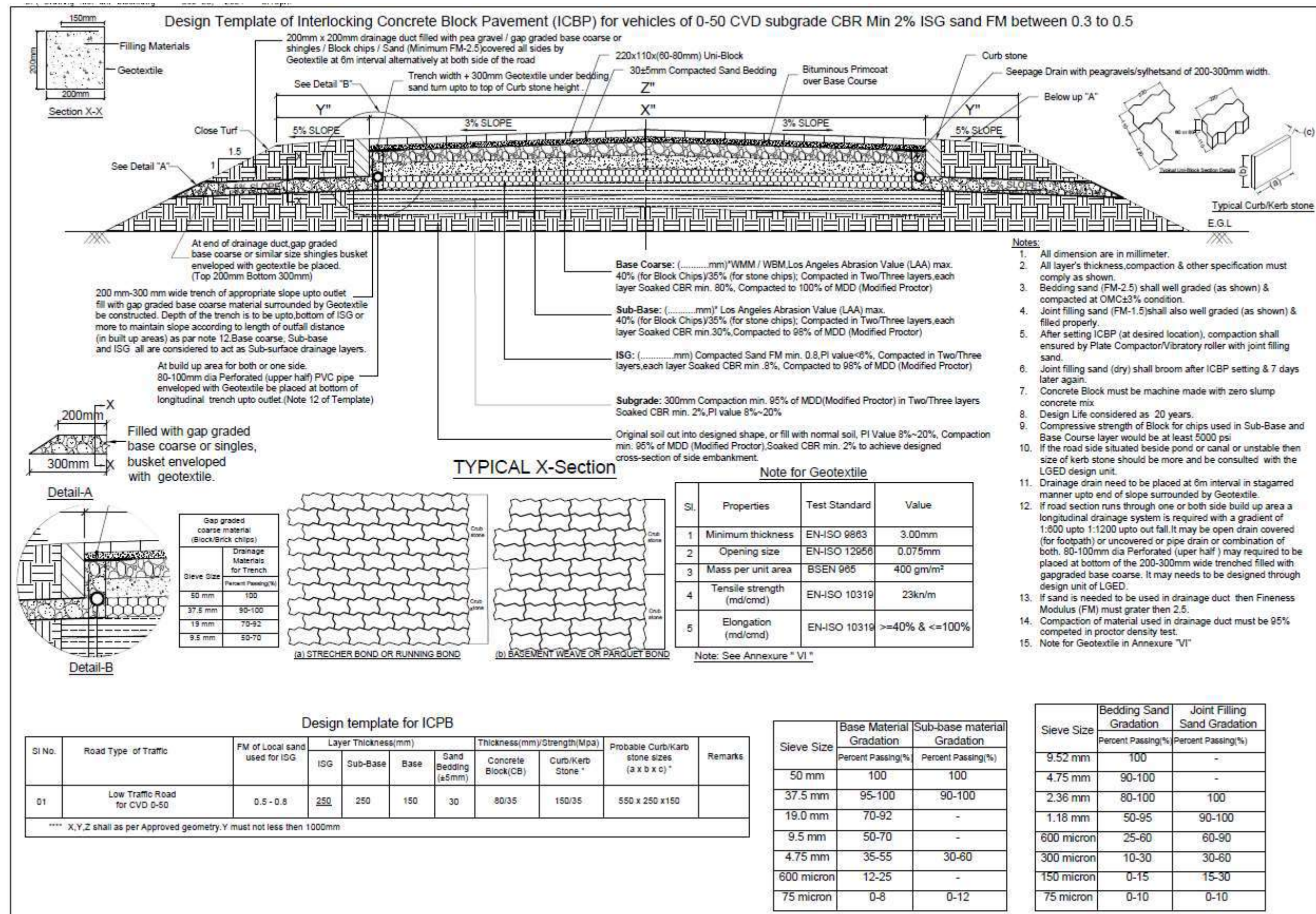
Figure 3.3: Design Template of Interlocking Concrete Block Pavement (ICBP) for vehicles of 0-50 CVD Subgrade CBR Minimum 2% ISG sand FM between 0.3-0.5
