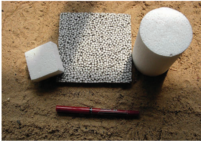
Figure 8. Geofoam examples
