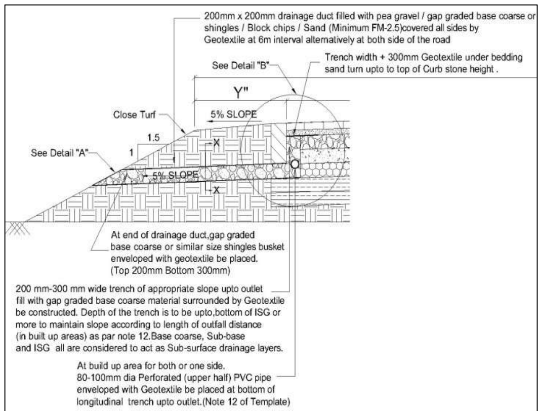
Figure 6.1: Sub Surface Drainage in a Block Pavement
