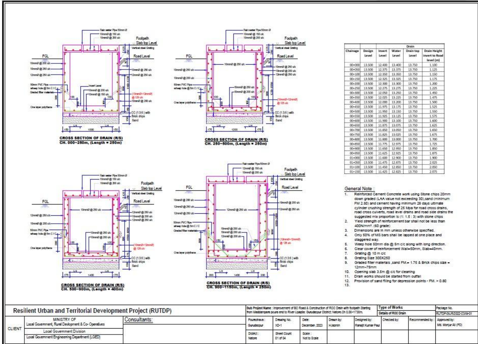
Figure 2.1.4: Cross-section of the Proposed Drainage Improvements
