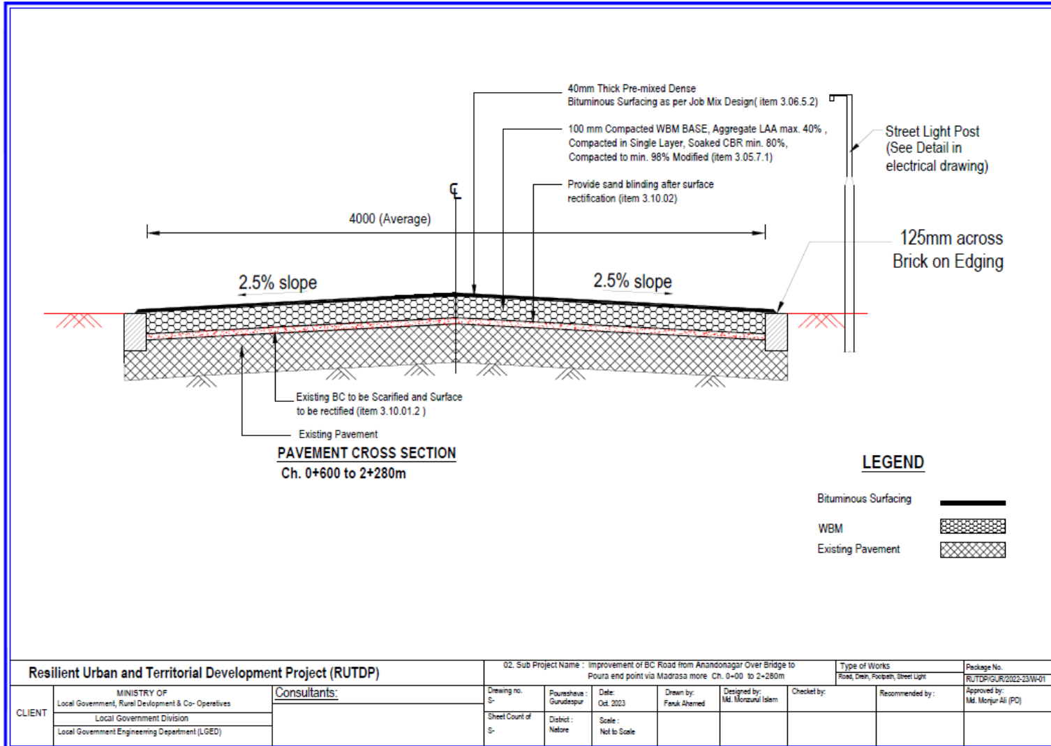
Figure 2.1.3: Cross-section, of the proposed BC road for the Pourashava
