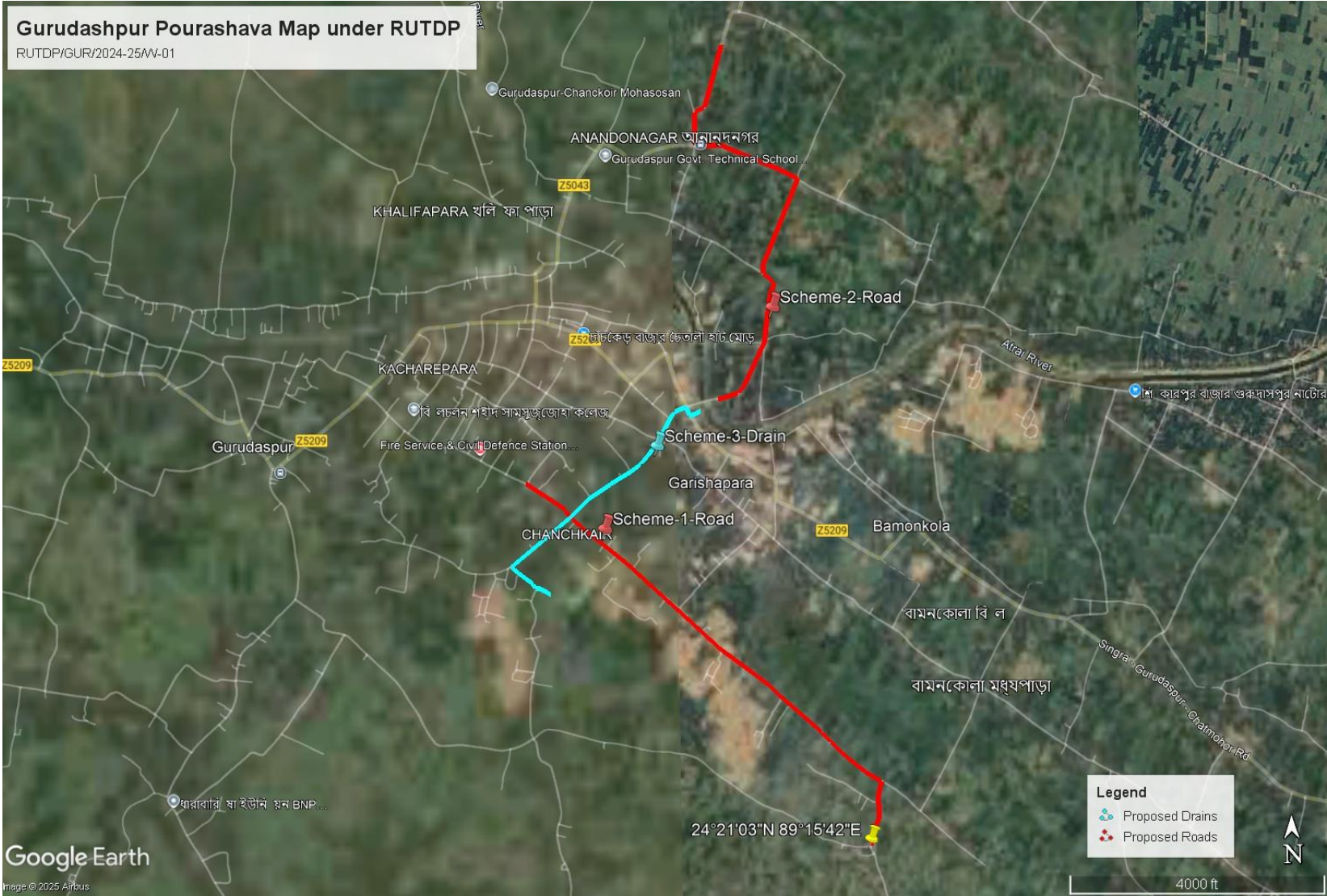
Figure 2.1.2: Topographic Features of the Subproject Area and its Adjoining Roads with Influence Zone
