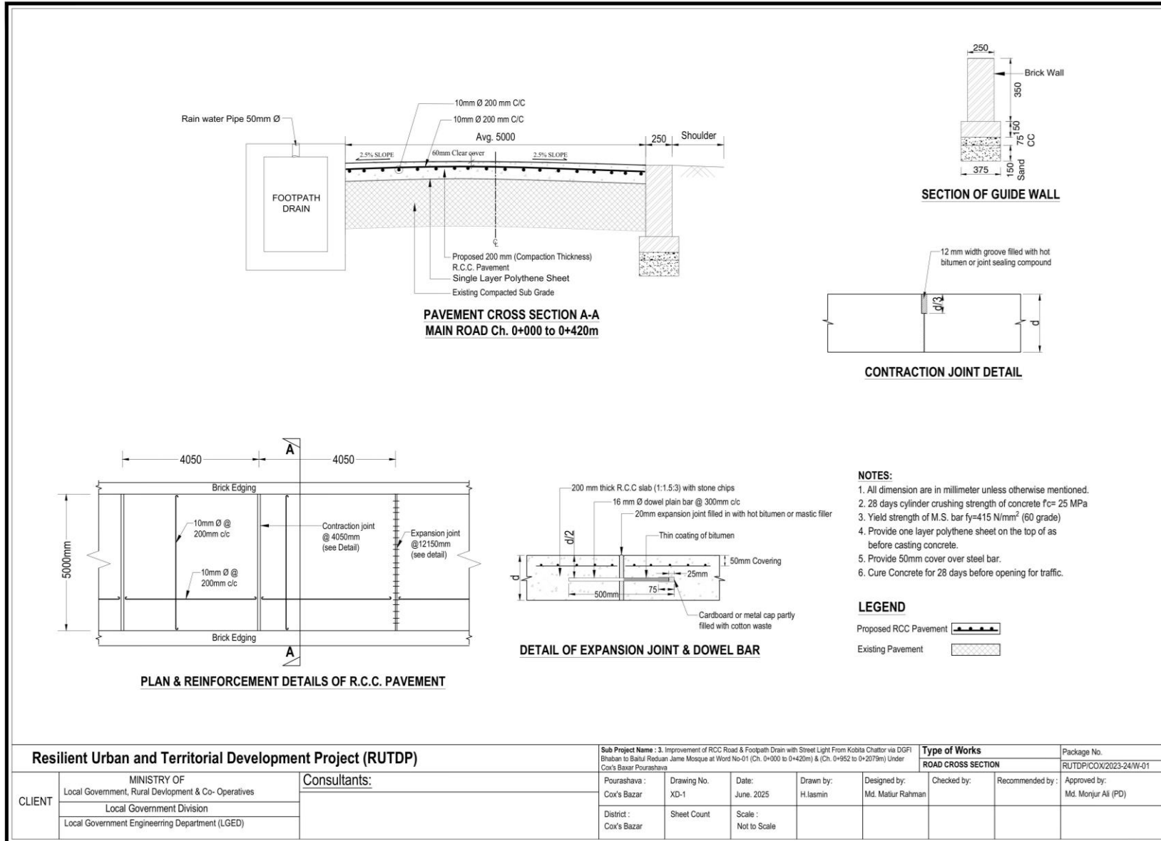
Figure 2.1.5: Cross-section, of the proposed RCC road for the Pourashava
