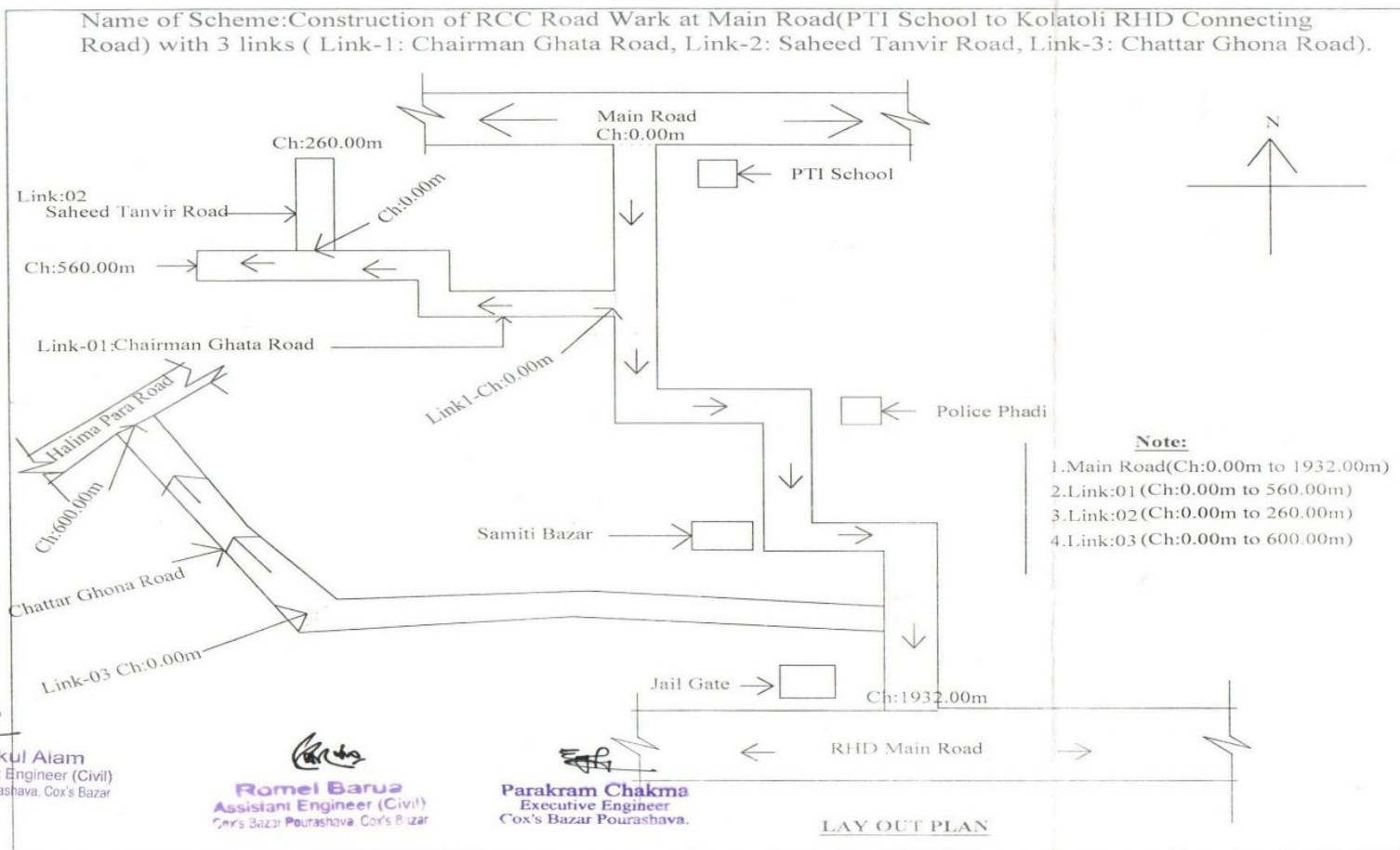
Figure 2.1.4: Zone Layout Plan of the Proposed Subproject Area (Drain) and its Adjoining Roads with Influence Zone
