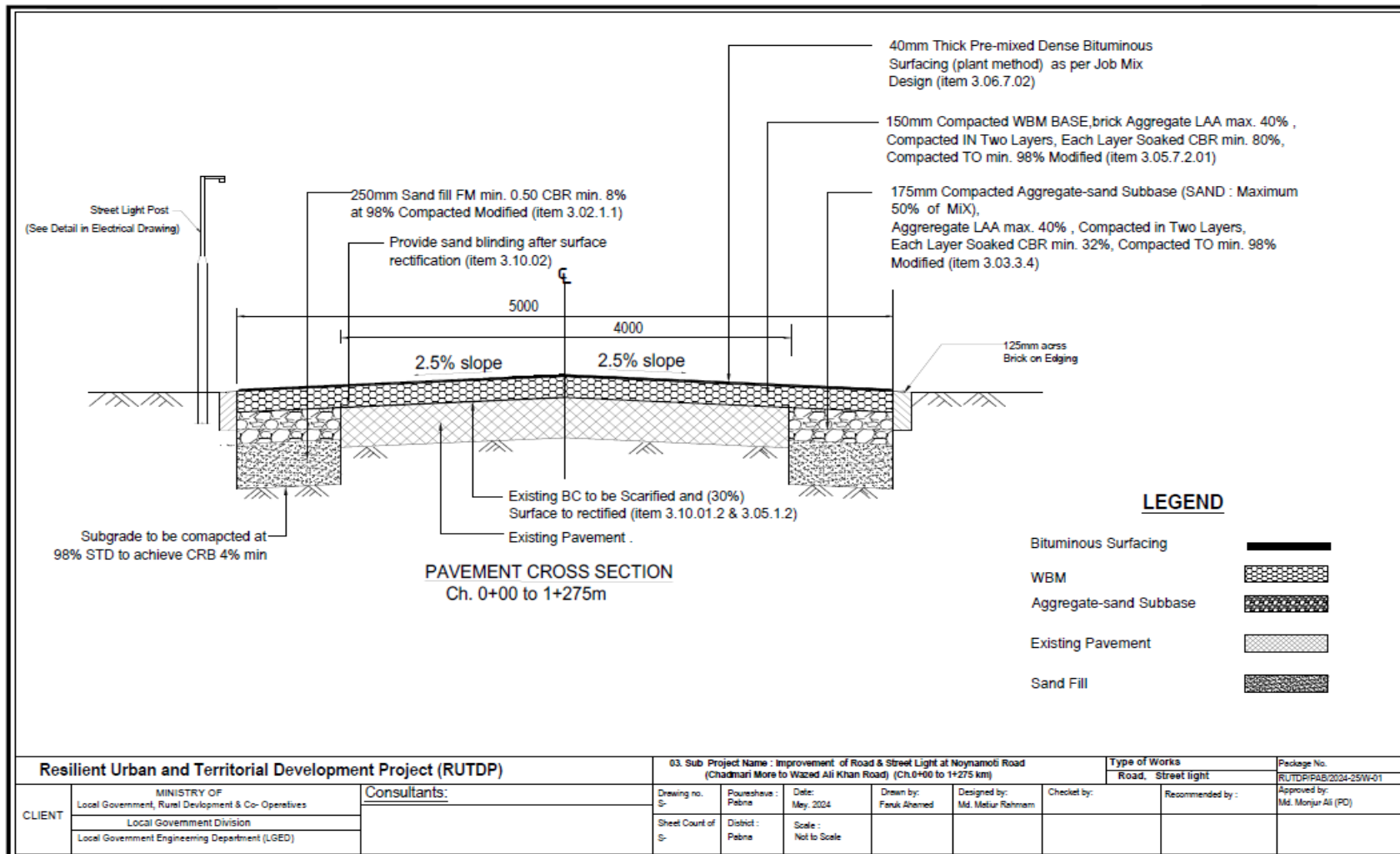
Figure 2.1.5: Cross-section of the proposed BC Road Improvements for the Pourashava
