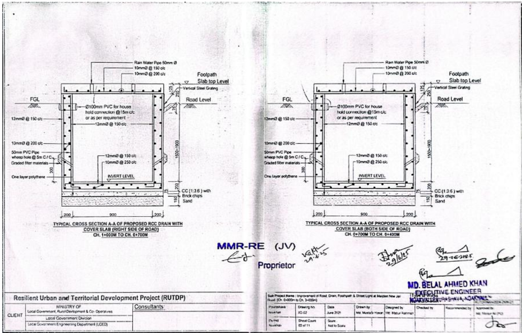
Figure 2.1.8: Cross-sections of the proposed RCC Drain for the Pourashava
