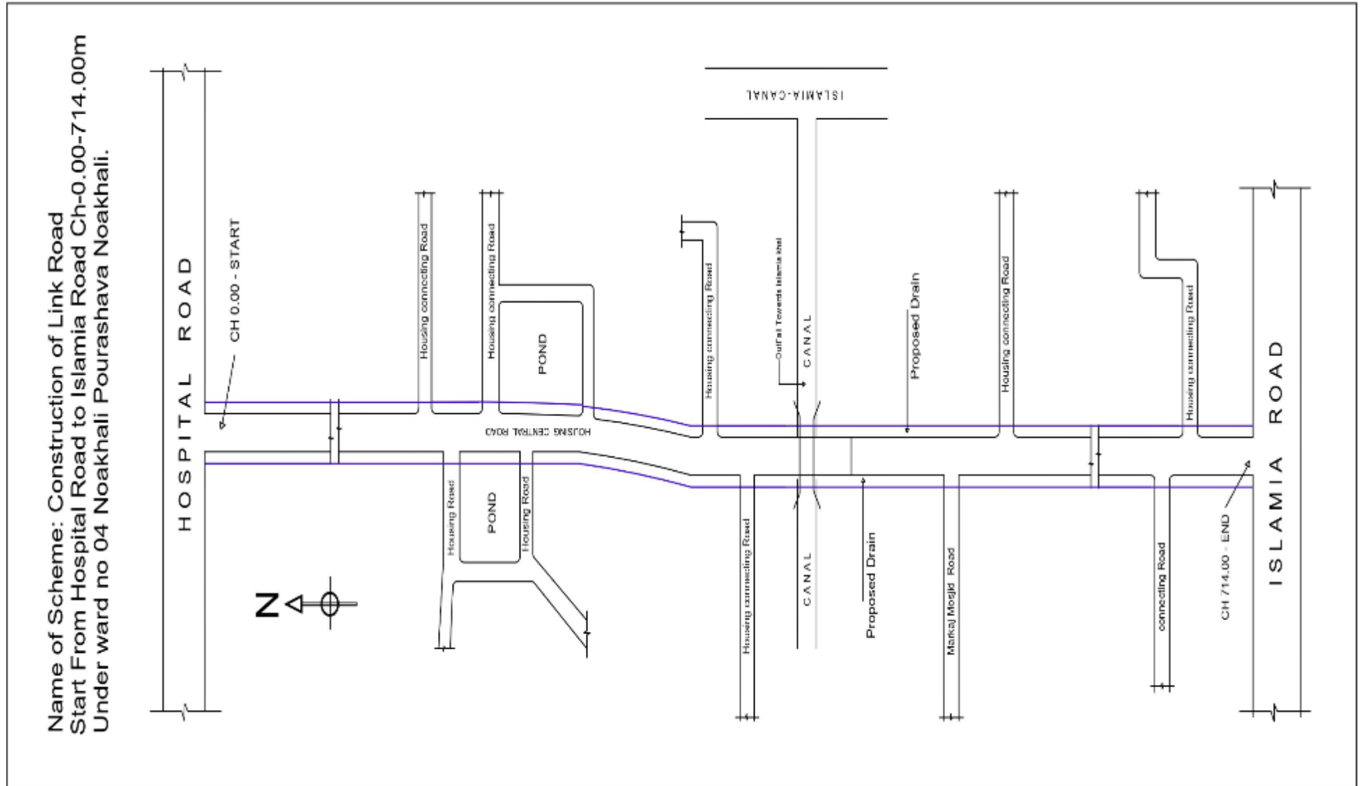
Figure 2.1.6: Layout Plan for the Proposed Subproject Area at Link Road of Noakhali Sadar Hospital Road
