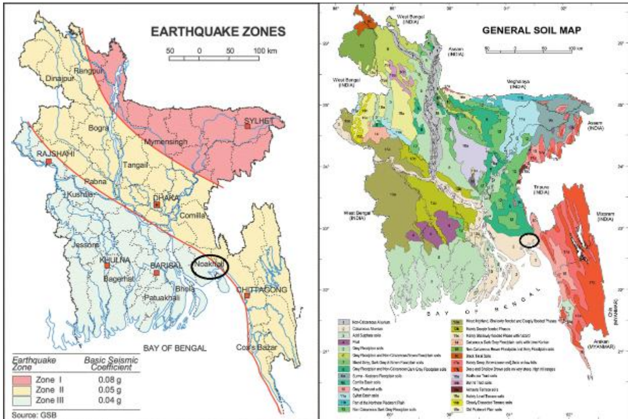
Figure 3.1.1: Location of Noakhali Pourashava in Earthquake Zoning map of Bangladesh [Source: GSB, 1978] and general soil map of Bangladesh [Source: BARC, 2005] (the black circle denotes Noakhali Pourashava)
