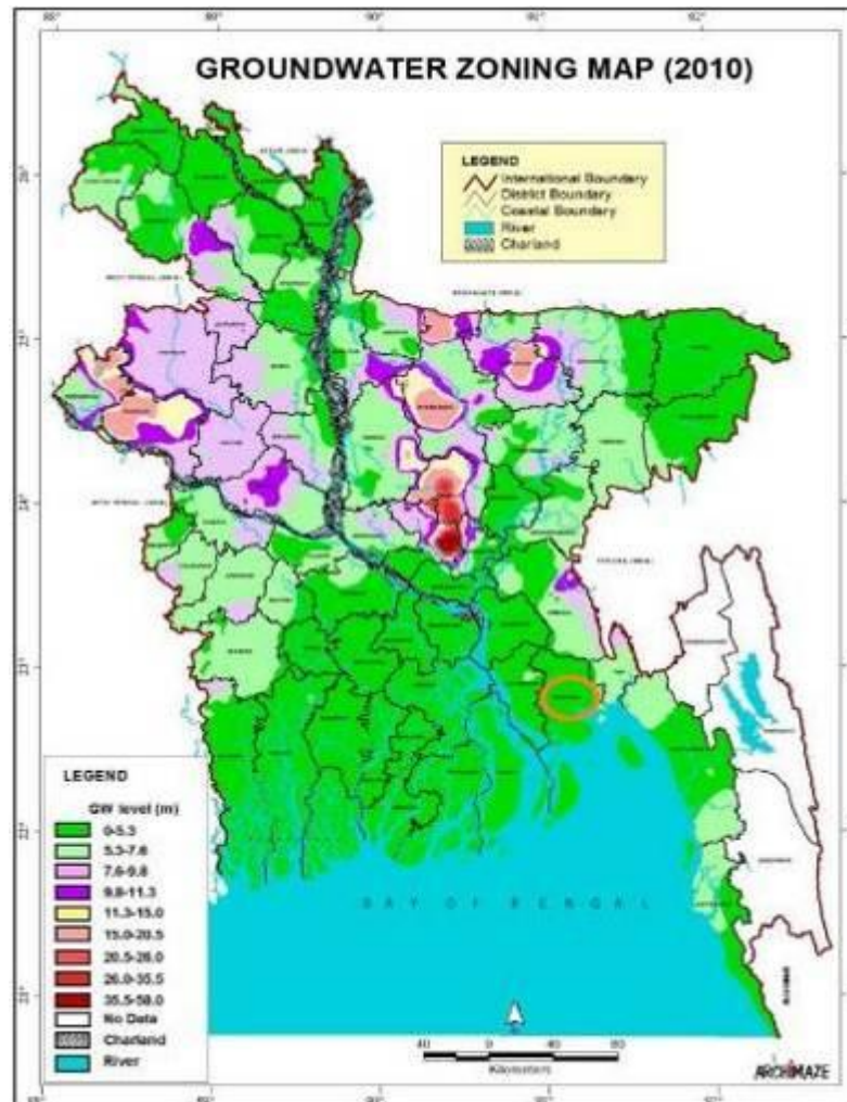
Figure 3.1.2: Location of Noakhali Pourashava in Groundwater Zoning Map of Bangladesh [Source: BADC, 2010] (the red circle denotes Noakhali Pourashava)
