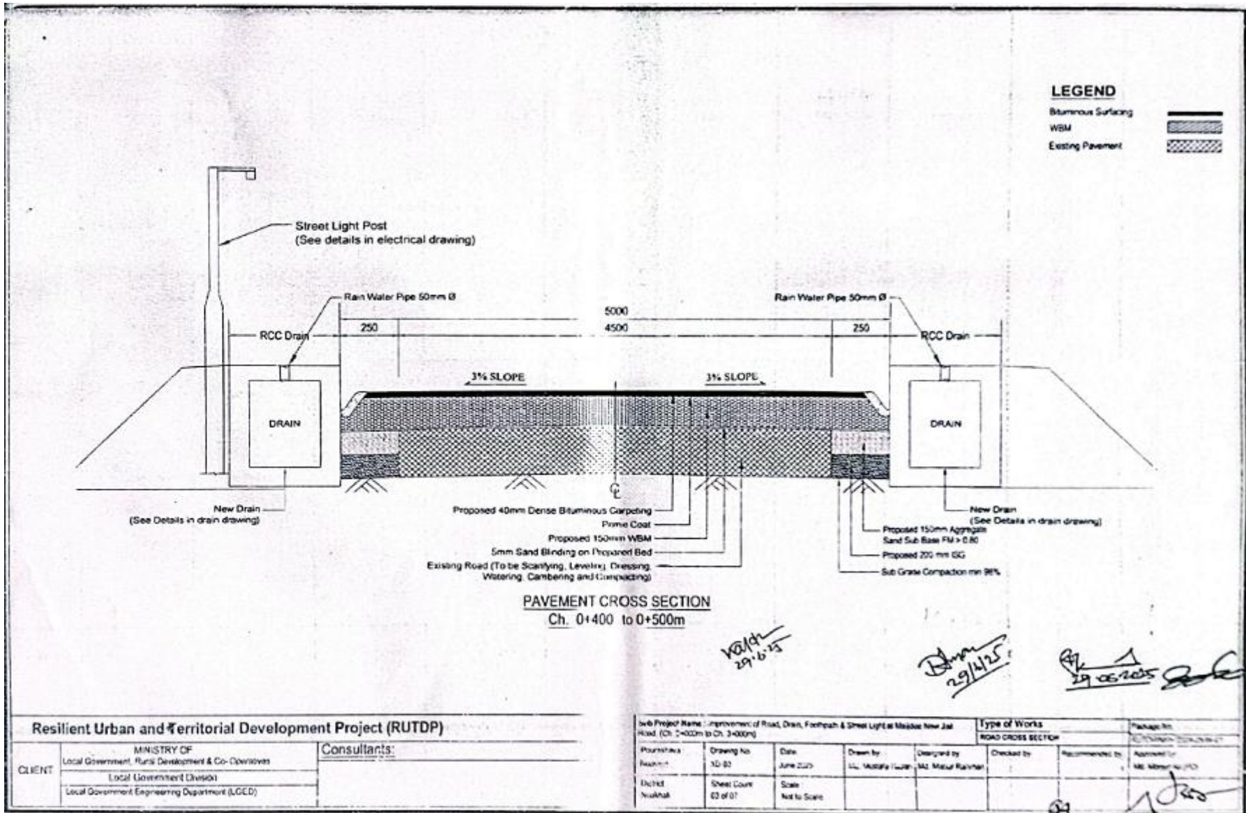
Figure 2.1.7: Cross-sections of the proposed BC road for the Pourashava
