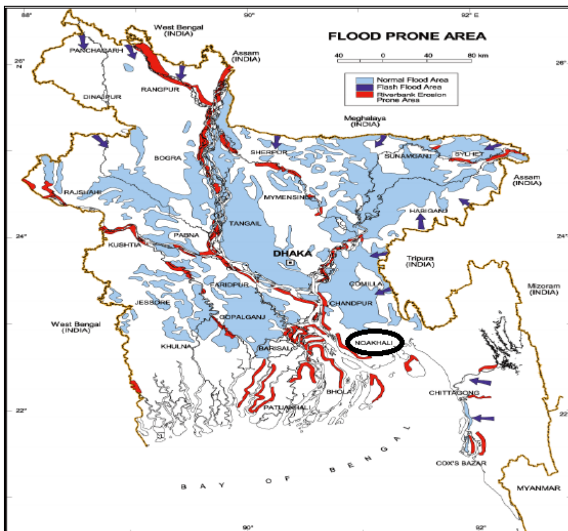
Figure 3.1.3: Location of Noakhali Pourashava in Flood Zone Map of Bangladesh [Source: BMD]
