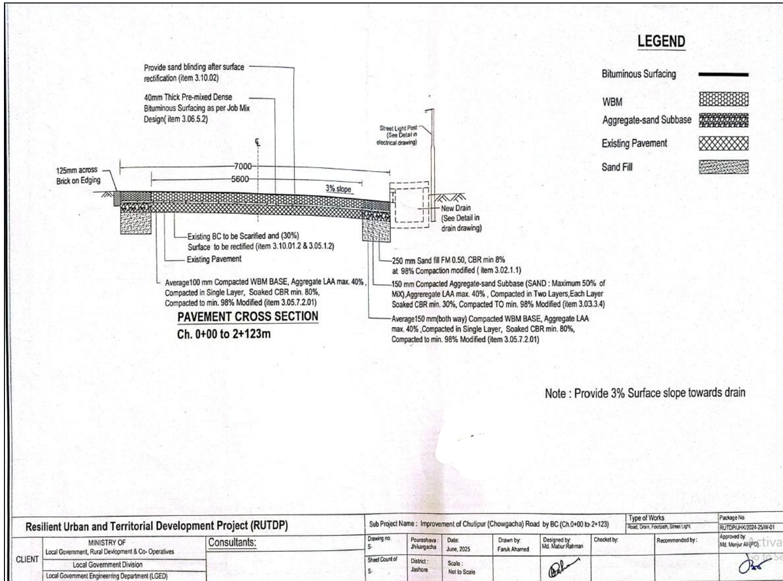
Figure 2.1.7: Cross Section of the BC road of the subproject
