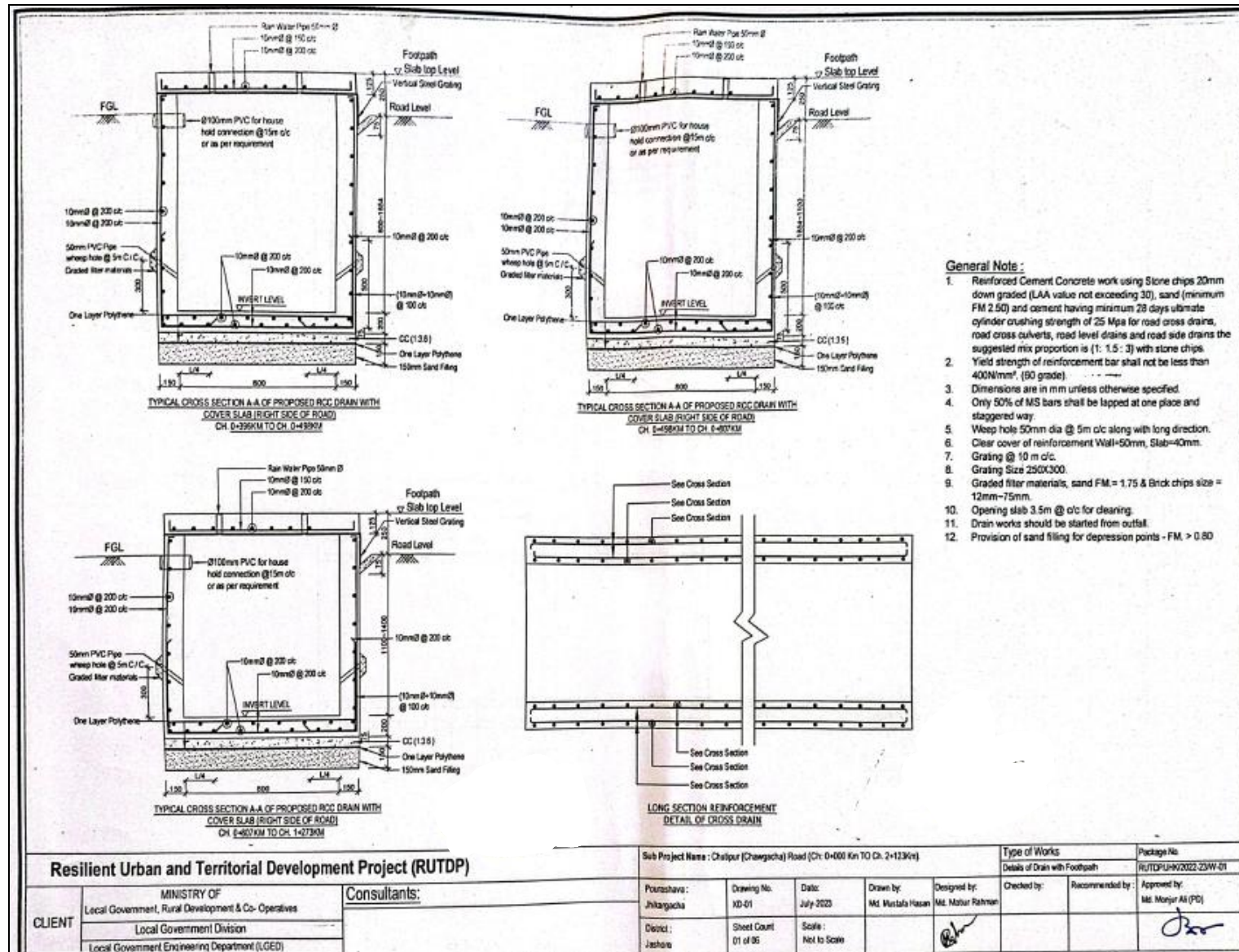
Figure 2.1.6: Cross Section of the RCC Drain of the subproject
