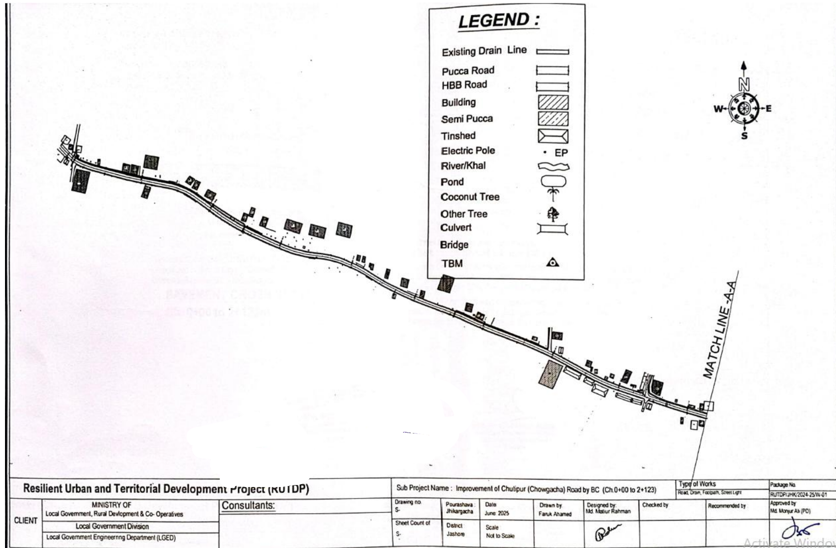
Figure 2.1.5: Zone Layout Plan of the Proposed Subproject Area (Drain) and its Adjoining Roads with Influence Zone
