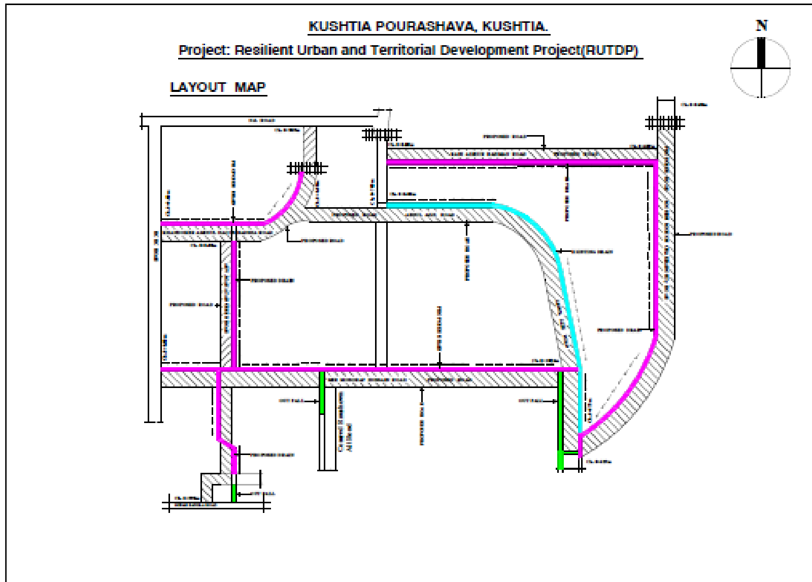
Figure 2.1.4: Layout Plan for the proposed Subproject area and its adjoining roads
