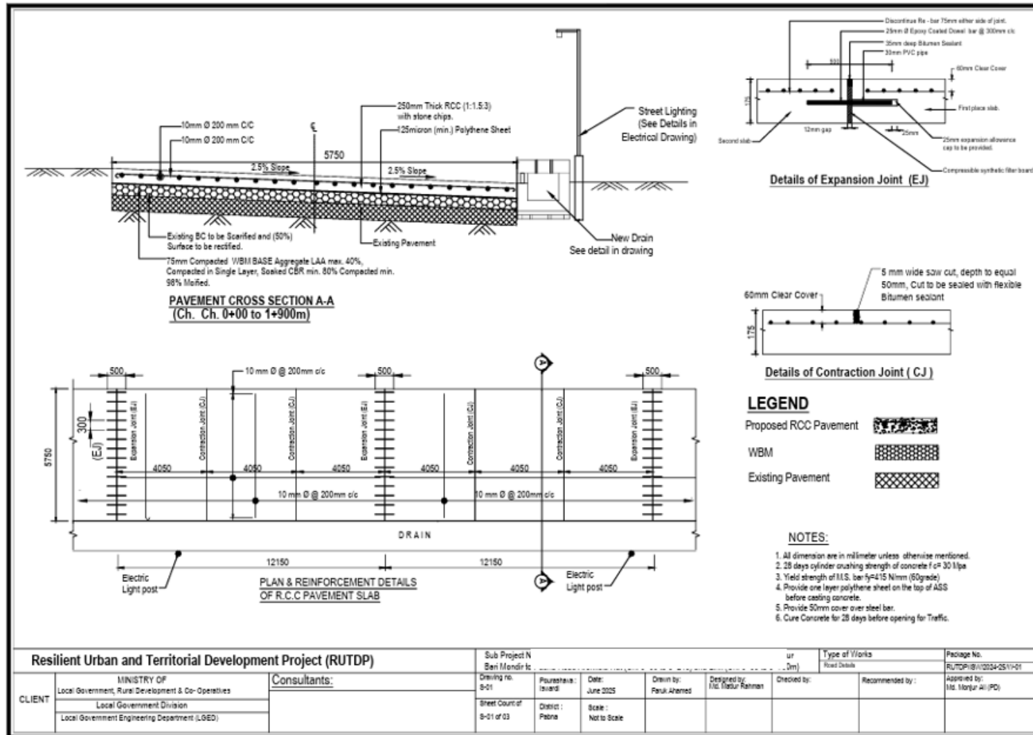
Figure 2.1.5: Cross Section of the Proposed Roads
