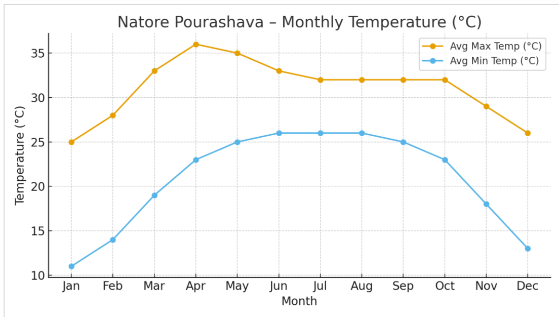
Figure 3.1.2: Monthly Temperature (°C)
