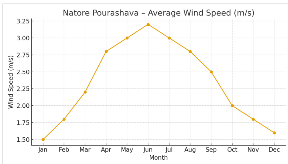
Figure 3.1.5: Wind Speed (m/s)
