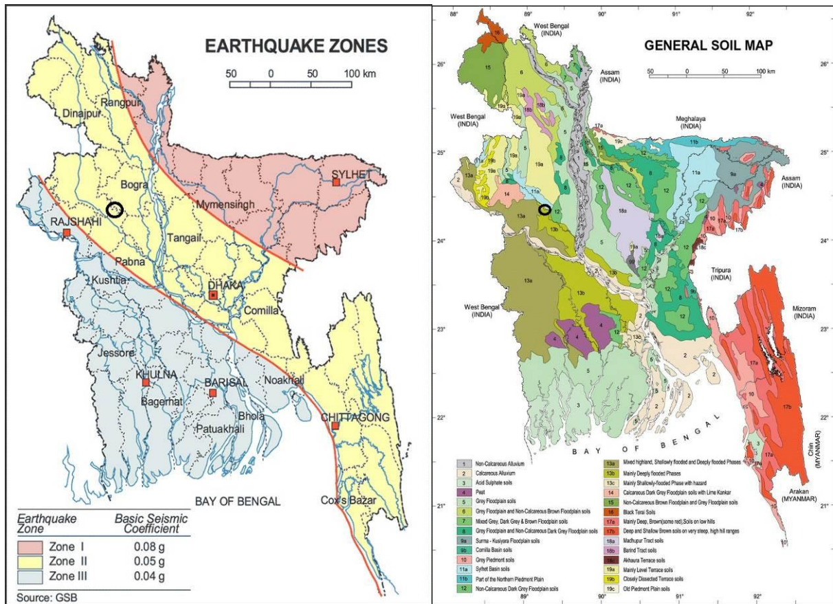
Figure 3.1.1: Location of Natore Pourashava in Earthquake Zoning map of Bangladesh [Source: GSB, 1978] and general soil map of Bangladesh [Source: BARC, 2005] (the Black circle denotes Natore Pourashava)
