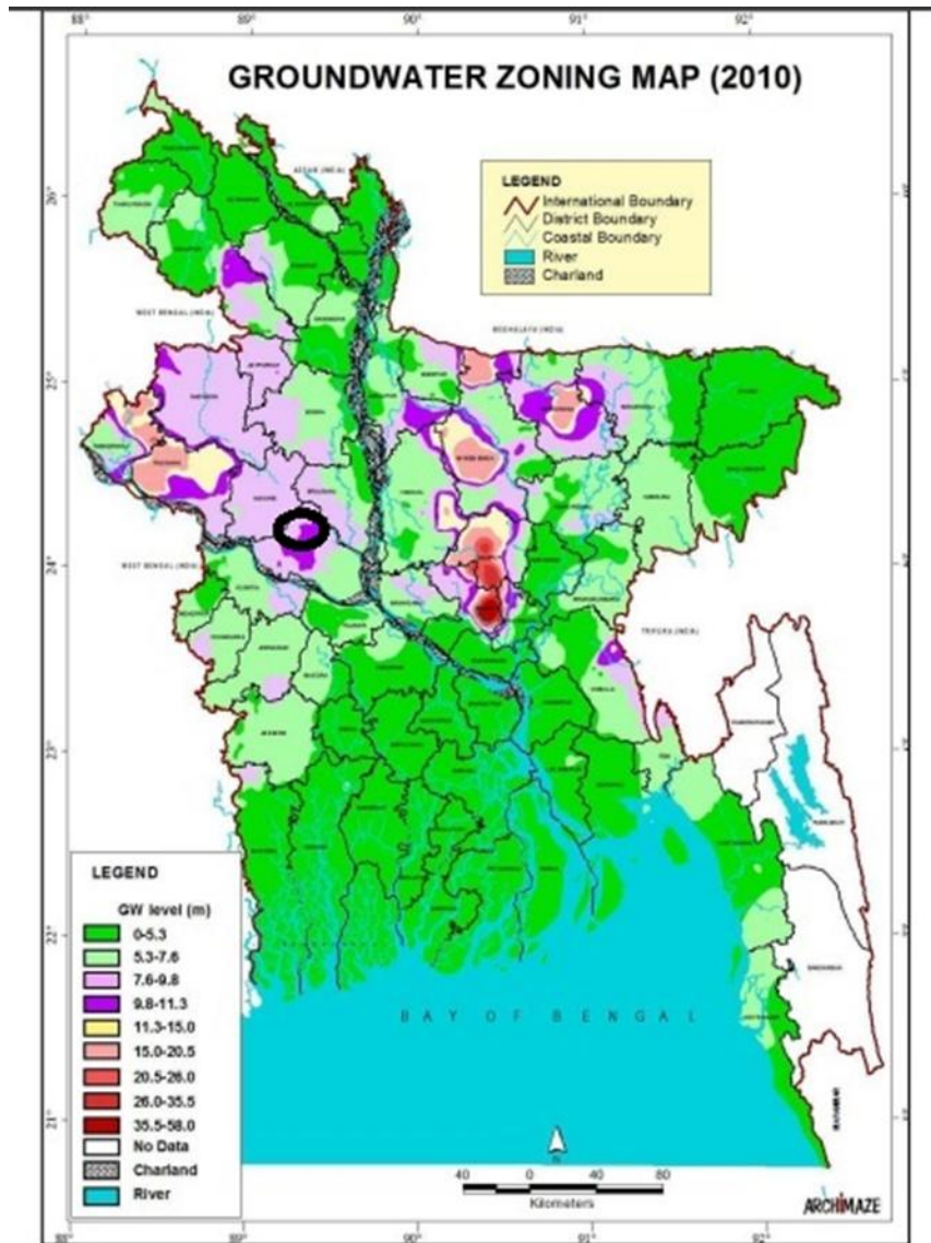
Figure 3.1.6: Location of Natore Pourashava in Groundwater Zoning Map of Bangladesh [Source: BADC, 2010] (the black circle denotes Natore Pourashava)
