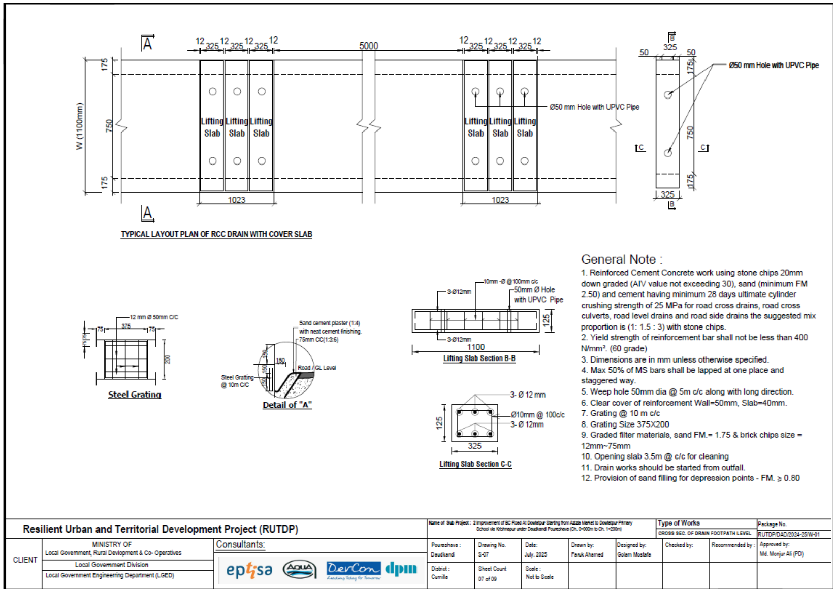
Figure 2.1.3: Cross-section of the Proposed Drainage Improvements
