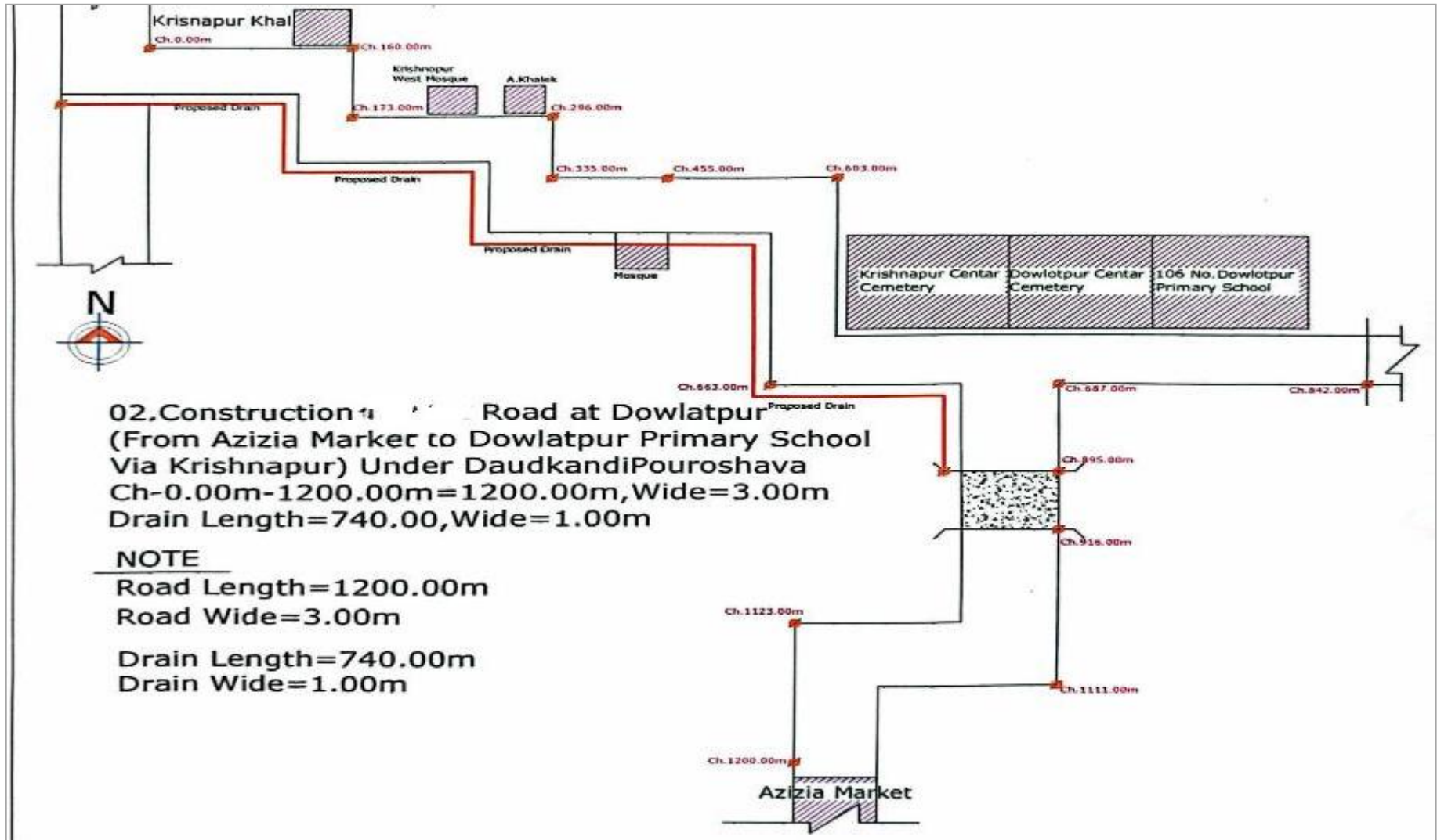
Figure 2.1.4: Layout Plan for the Proposed Subproject Area at Dowlatpur starting from Azizia Market to Dowlatpur Primary School via Krishnapur
