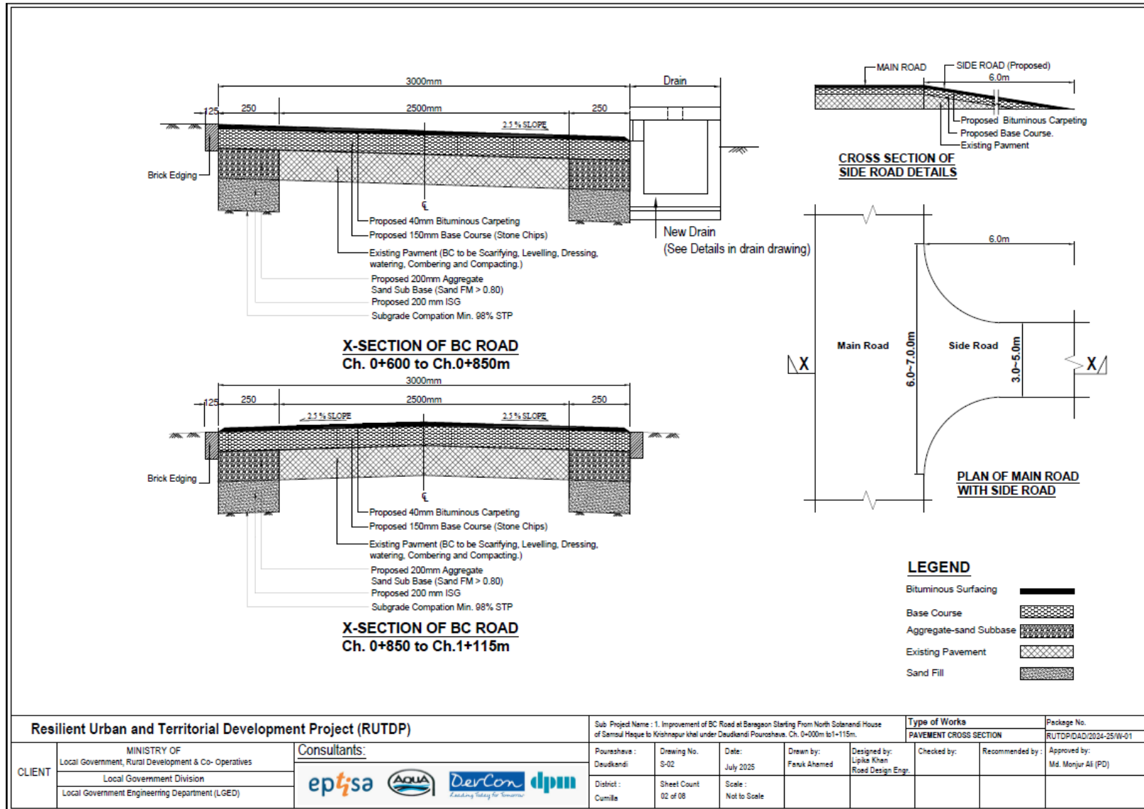
Figure 2.1.2: Cross-section, of the proposed BC Road for the Pourashava
