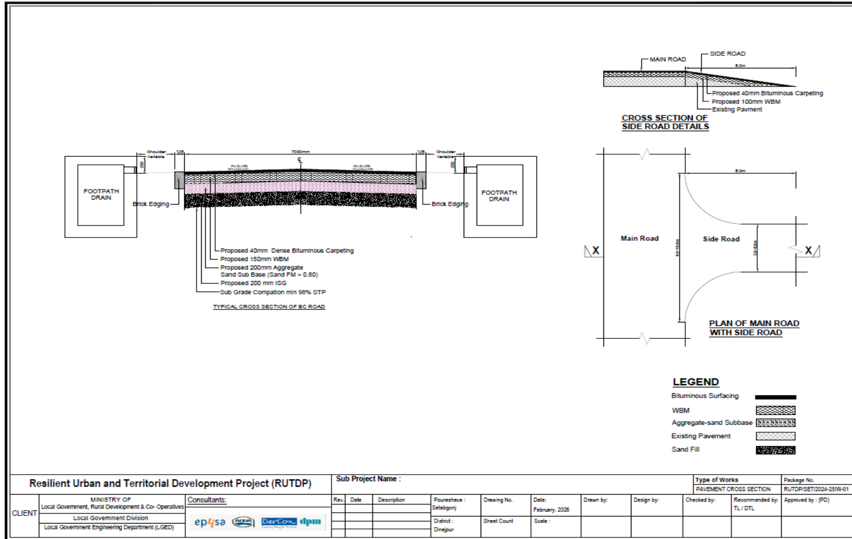
Figure 2.1.6: Typical Cross Section of BC road of the Subproject
