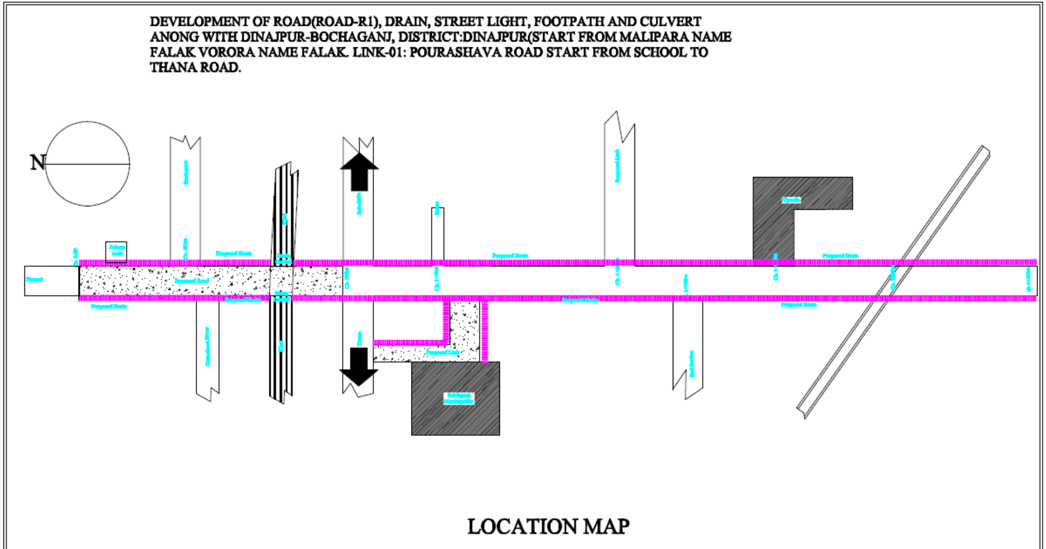
Figure 2.1.4: Layout Plan of the Proposed Subproject Area (Road) and its Adjoining Roads with Influence Zone
