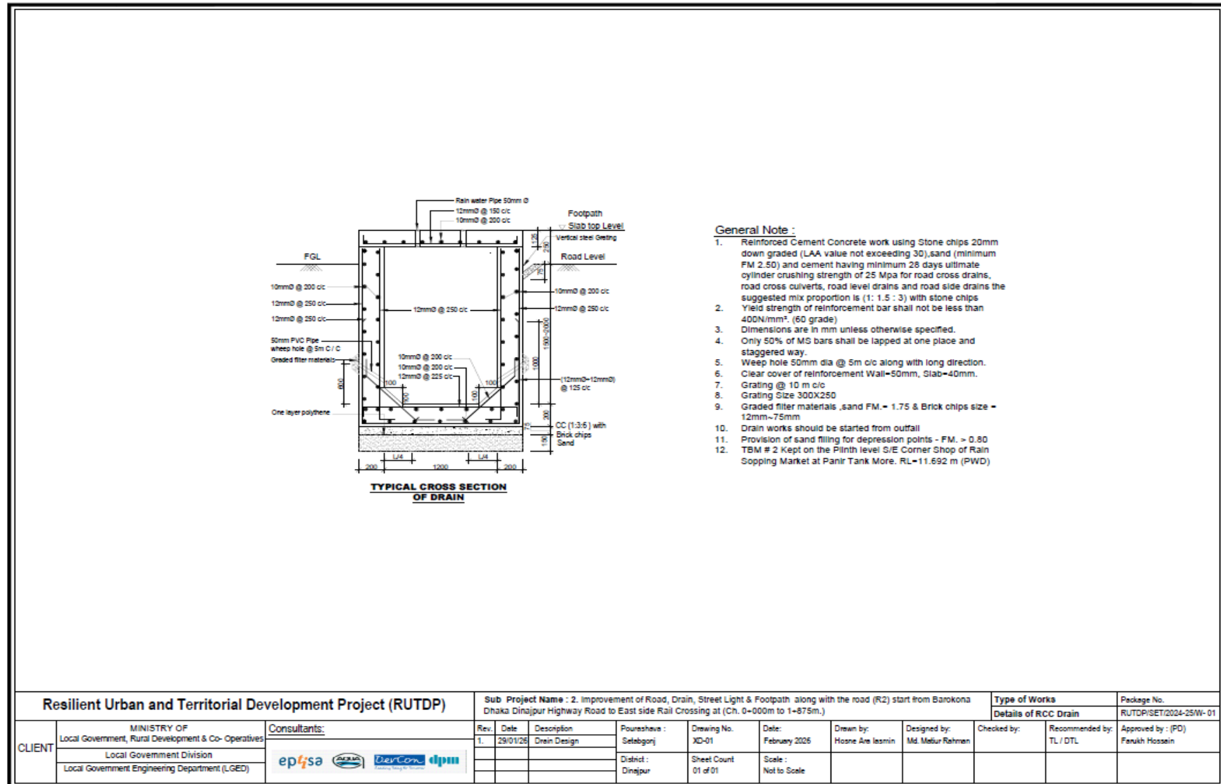
Figure 2.1.7: Typical Cross Section of RCC Drain of the Subproject
