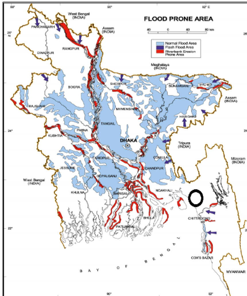
Figure 3.1.3: Location of Mirsharai Pourashava in Flood Zone Map of Bangladesh [Source: BMD]
