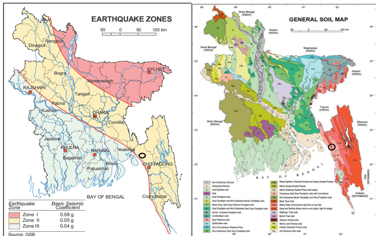
Figure 3.1.1: Location of Mirsharai Pourashava in Earthquake Zoning map of Bangladesh [Source: GSB, 1978] and general soil map of Bangladesh [Source: BARC, 2005] (the black circle denotes Mirsharai Pourashava)
