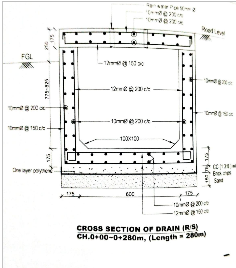
Figure 2.1.4: Cross Section of RCC Drain of the Subproject
