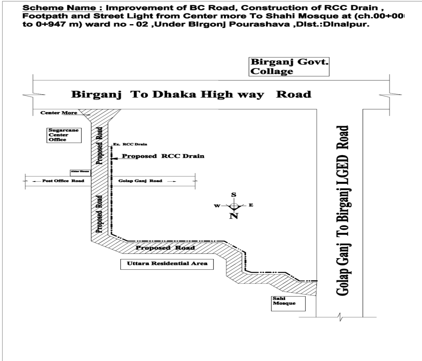
Figure 2.1.5: Layout Plan for the proposed Subproject area (Road-3) and its adjoining roads
