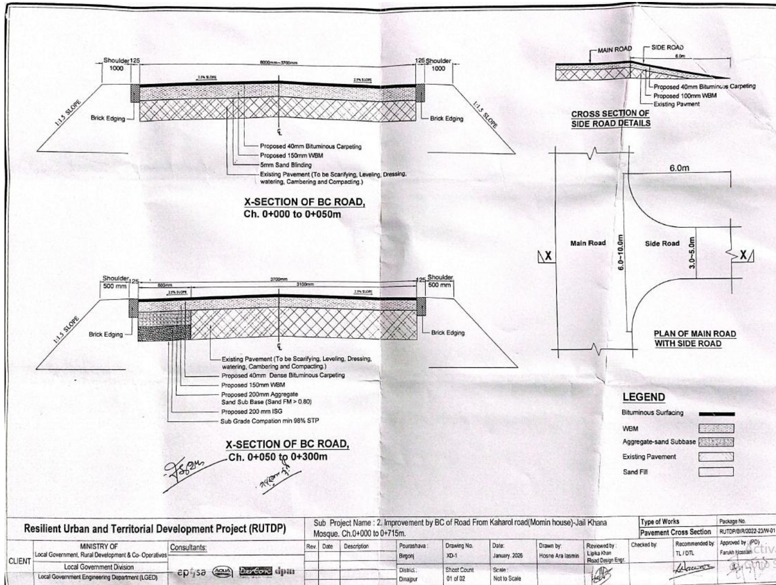
Figure 2.1.7: Cross-section of the BC Road of the proposed Subproject area
