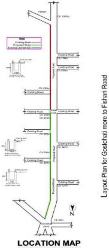
Figure 2.1.5: Zone Layout Plan of the Proposed Subproject Area (Road) and its Adjoining Roads with Influence Zone
