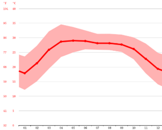
Figure 3.1.3: Climate Graph // Average Temperature by Month of Naogaon Pourashava
