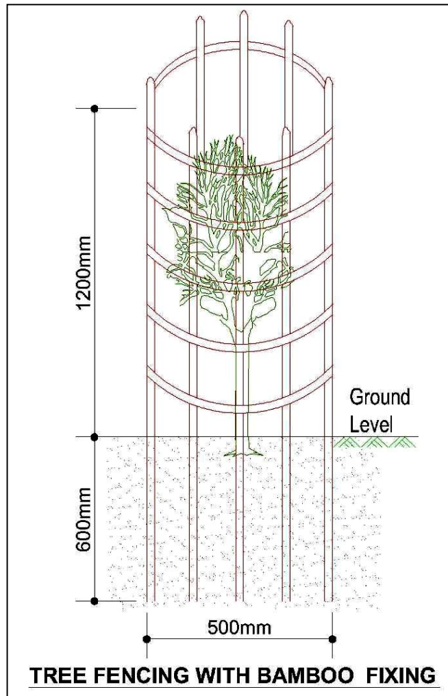
Figure 4.4.2.1: Drawing of Tree plantation procedure with bamboo fencing 4.4.3 Sand filling, back filling and Reinforced Cement Concrete works for RCC Culverts and Cross Drains
