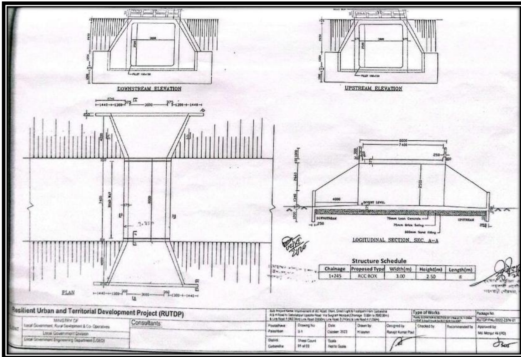
Figure 2.1.5: Cross Section of the Culvert of the Subproject
