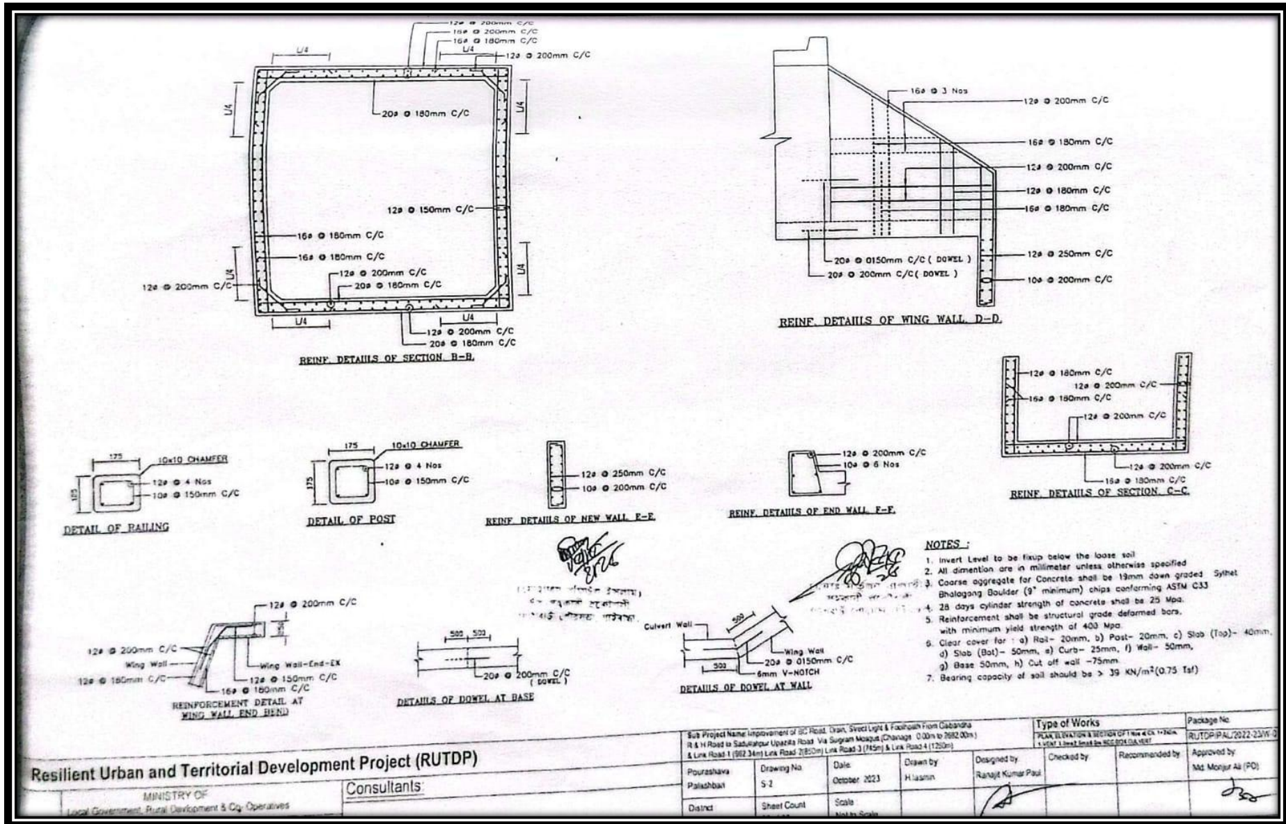
Figure 2.1.6: Cross Section of the RCC Drain of the Subproject
