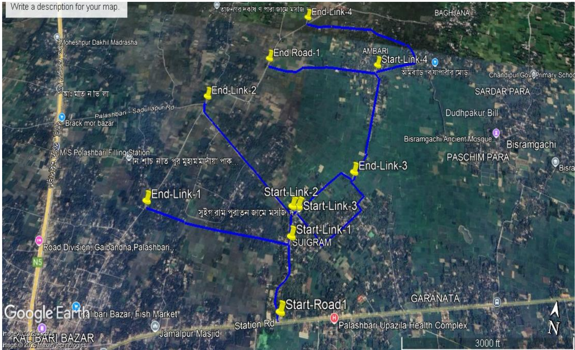
Figure 2.1.3: Topographical Features of the proposed Subproject area and its Adjoining Roads with Influence Zone
