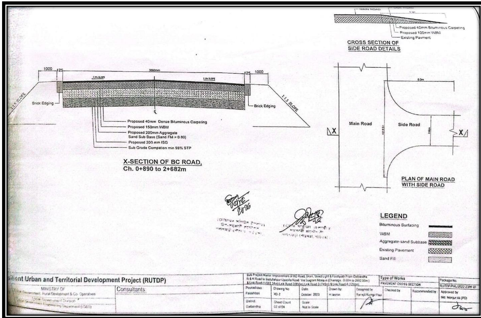
Figure 2.1.7: Cross Section of the BC ROAD of the Subproject
