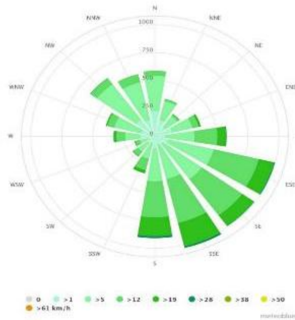
Figure 3.1.4: Wind rose Diagram in Project Area
