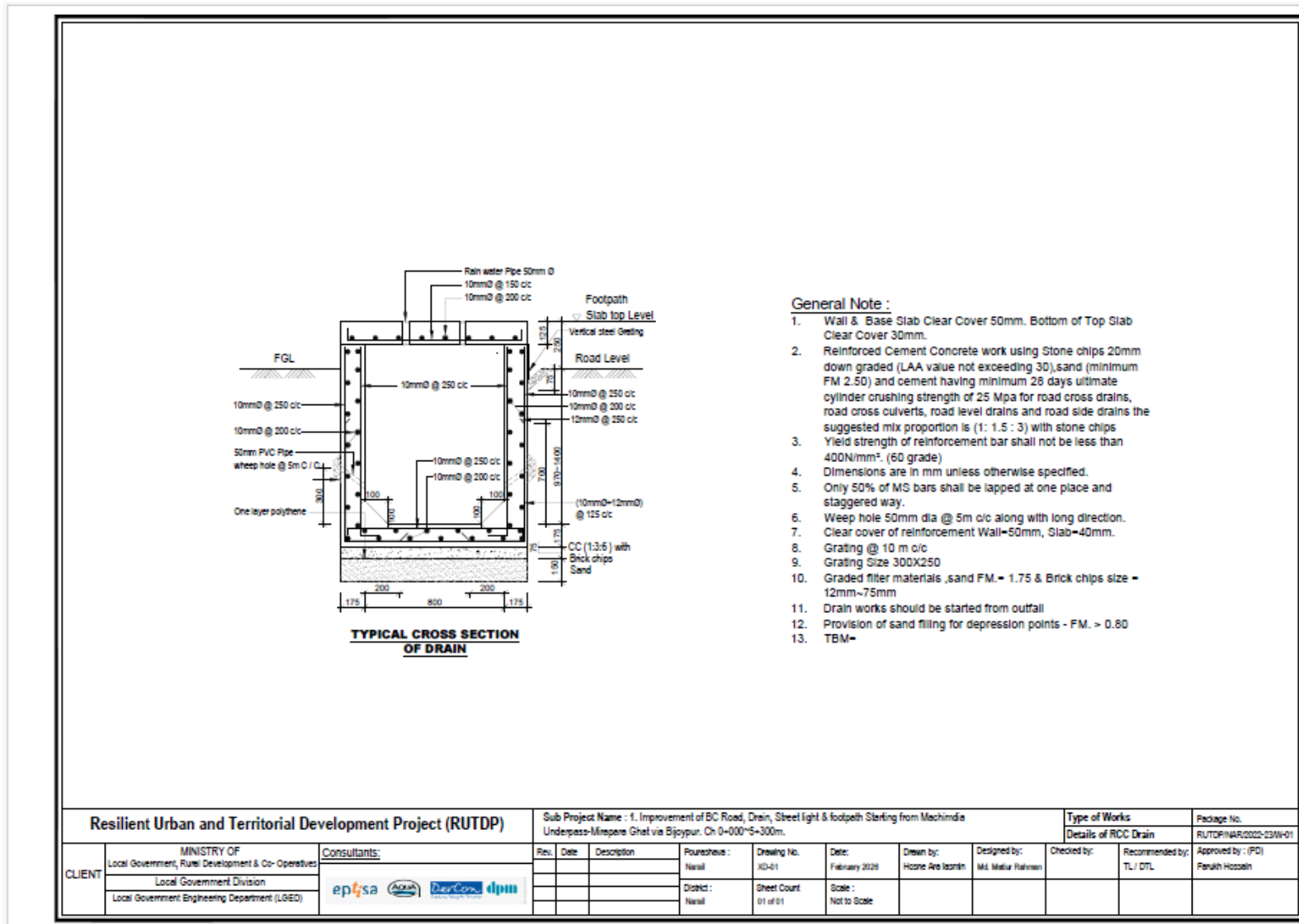
Figure 2.1.5: Cross Section for the proposed Subproject drains
