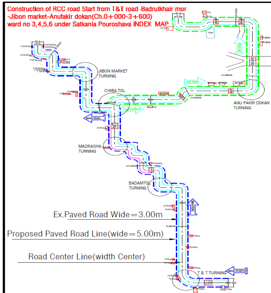
Figure 2.1.4: Layout Plan for the proposed Subproject Area from T & T Road-Badrul Khail Mor- Jibon Market-Anu Fakir Dokan and its adjoining roads
