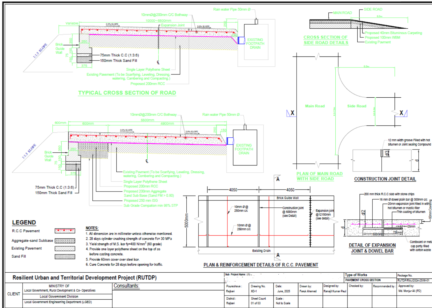
Figure 2.1.4: Cross Section for the proposed Subproject Area roads
