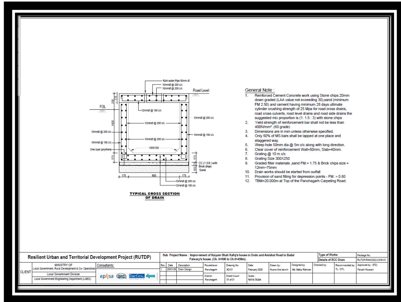
Figure 2.1.10: Cross Section of the RCC drain of the Subproject
