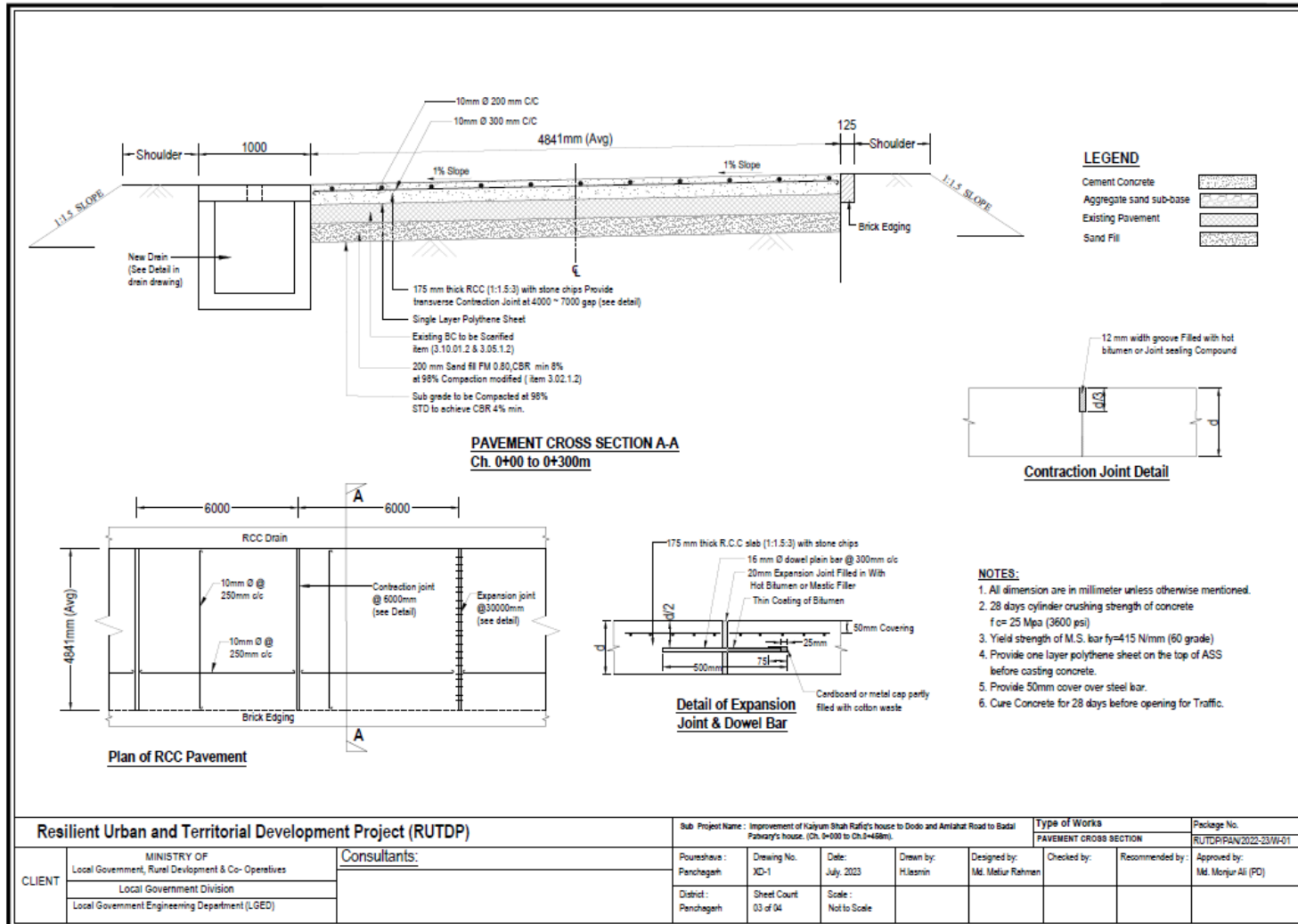
Figure 2.1.11: Cross Section of the BC Road of the Subproject
