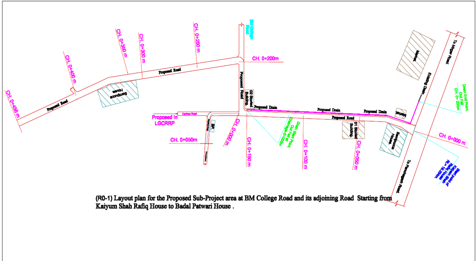
Figure 2.1.6: Layout Plan for the proposed Subproject area (R1) and its adjoining roads
