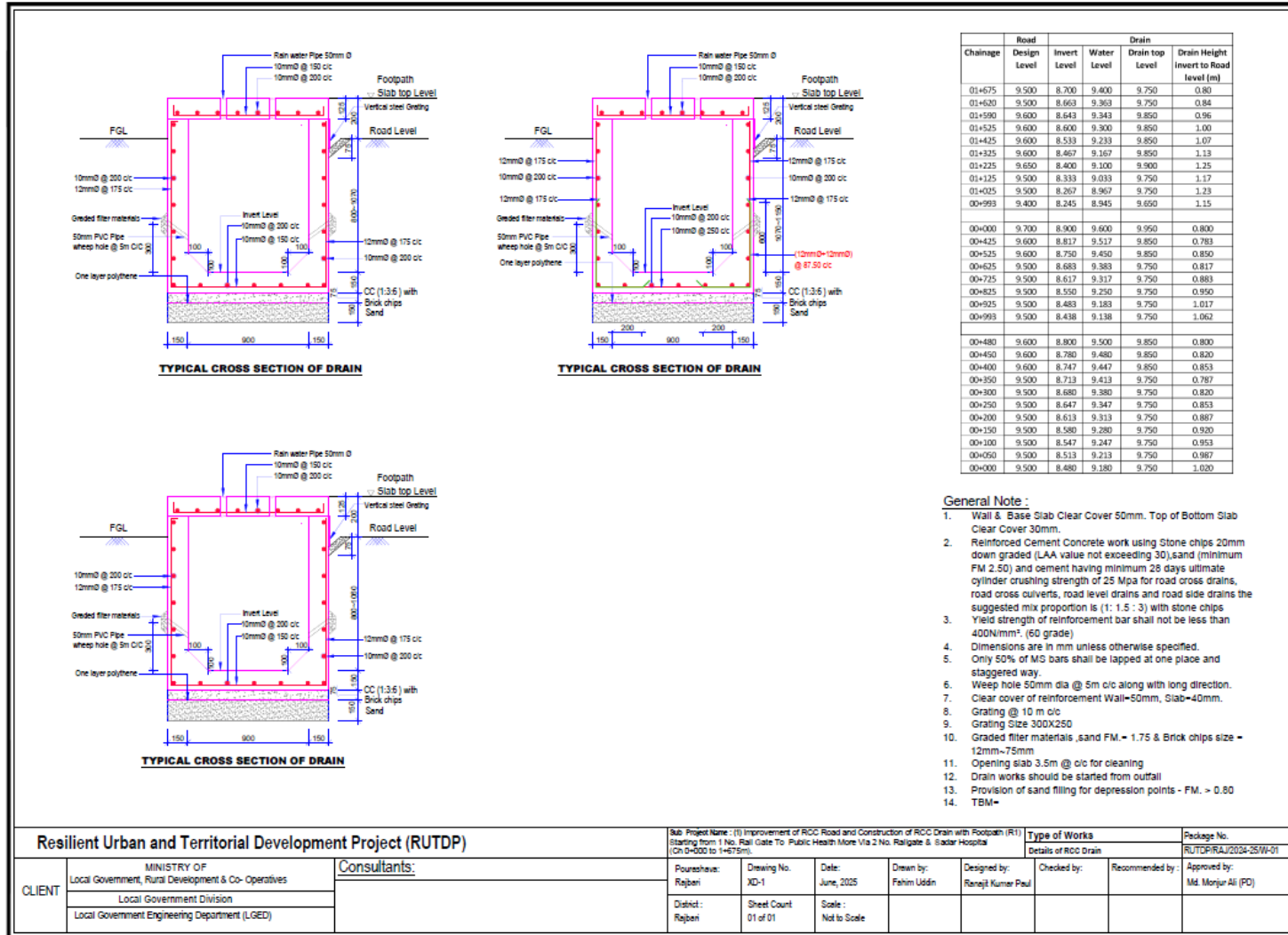
Figure 2.1.6: Cross Section of the RCC Darin of the Subproject
