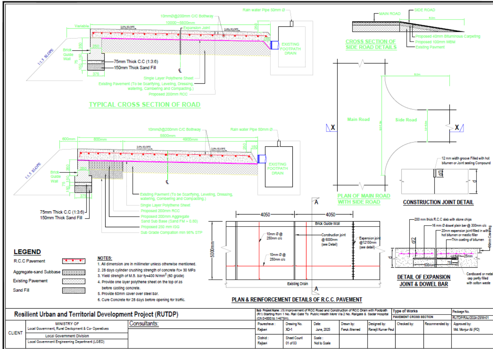
Figure 2.1.5: Cross Section of the RCC Pavement of the Subproject
